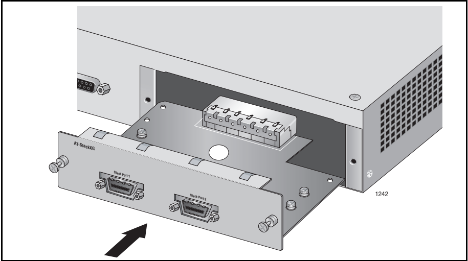
Figure 3. Installing the AT-StackXG Stacking Module
