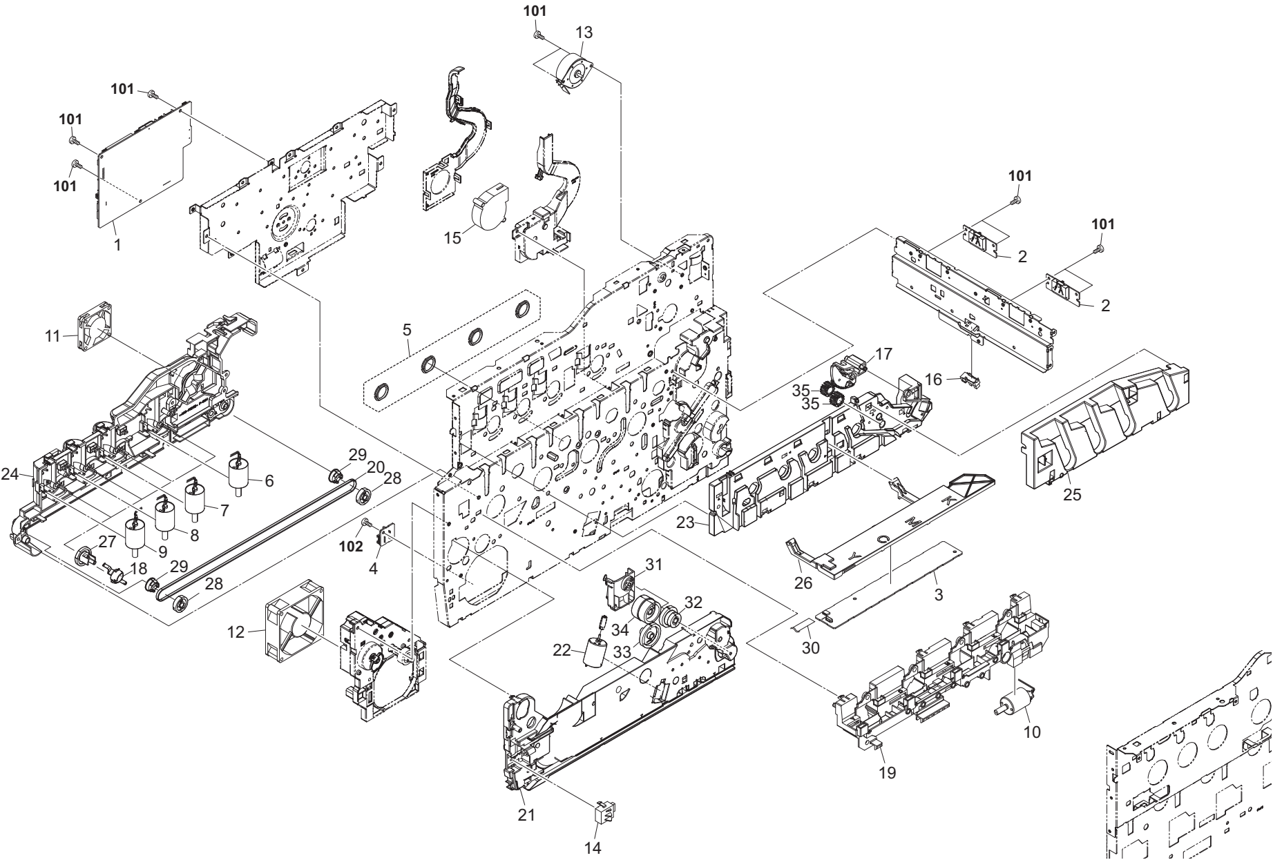
FIG. 12 Electrical Components 1
