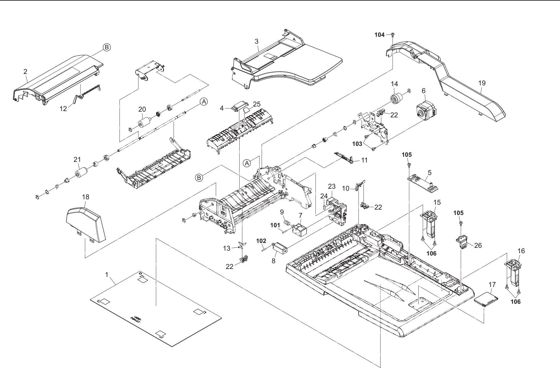
FIG. 16 Document Processor
