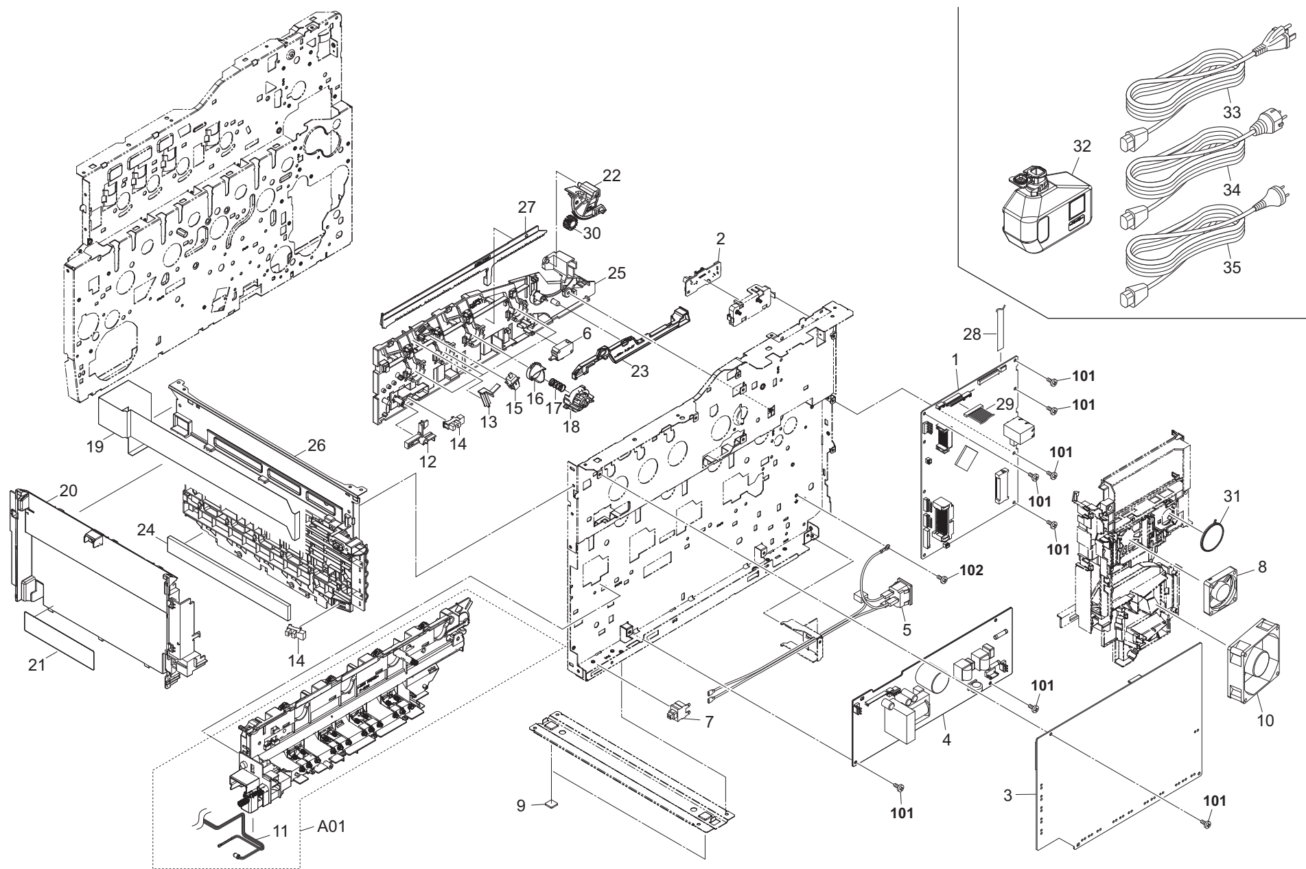
FIG. 13 Electrical Components 2
