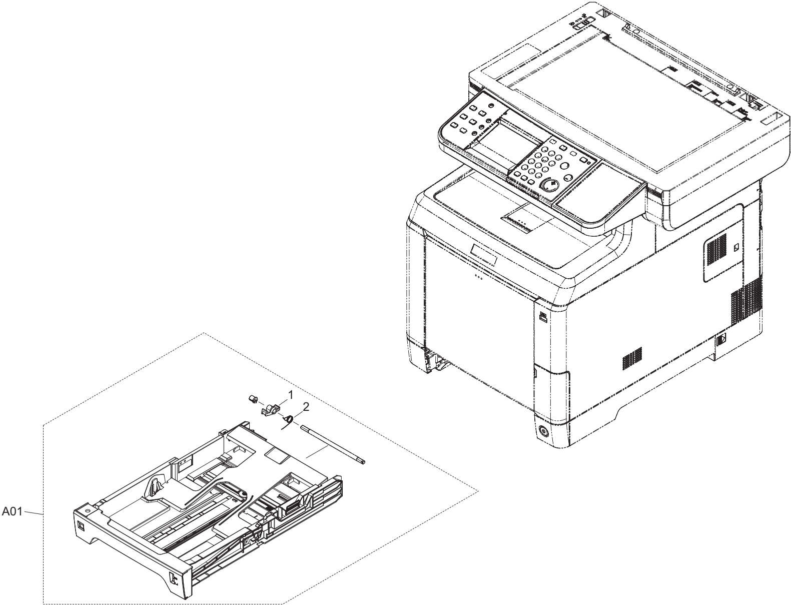
FIG. 2 Paper Cassette
