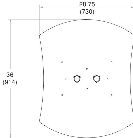
Base Detail
