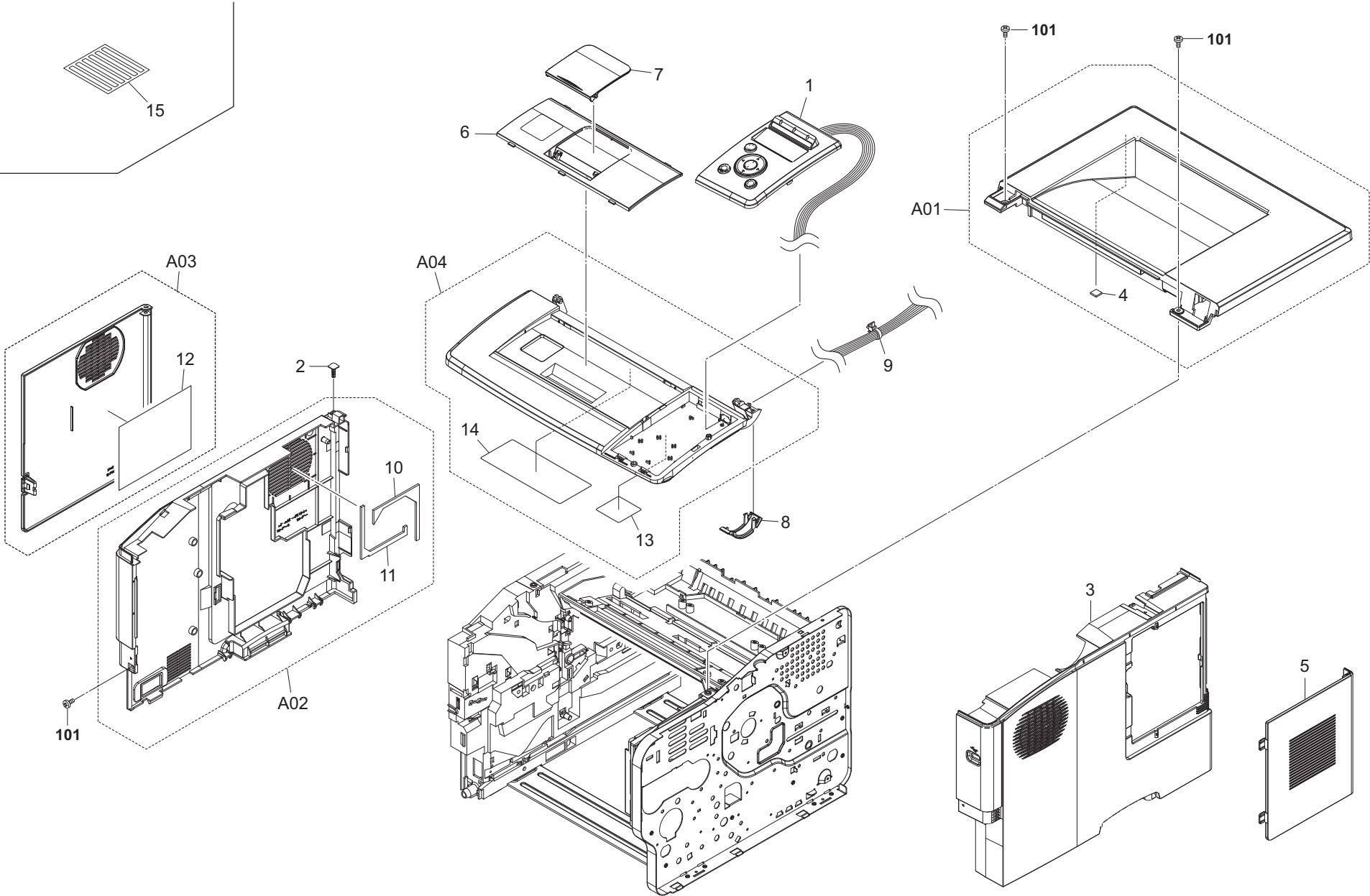
FIG. 1 Covers (FS-2020D)
