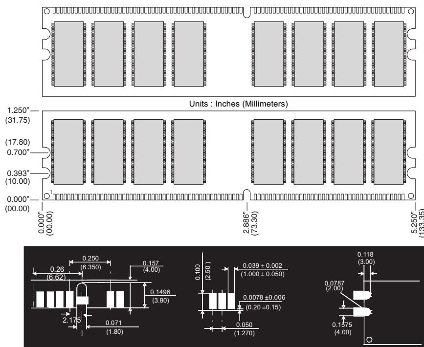
Figure 1: KVR400/512R 184-Pin DIMM
