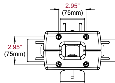
REAR MOUNTING HOLES
