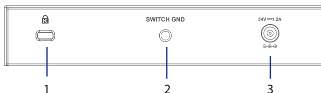
Figure 3: Rear panel connectors
