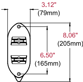
WALL PLATE DETAIL
