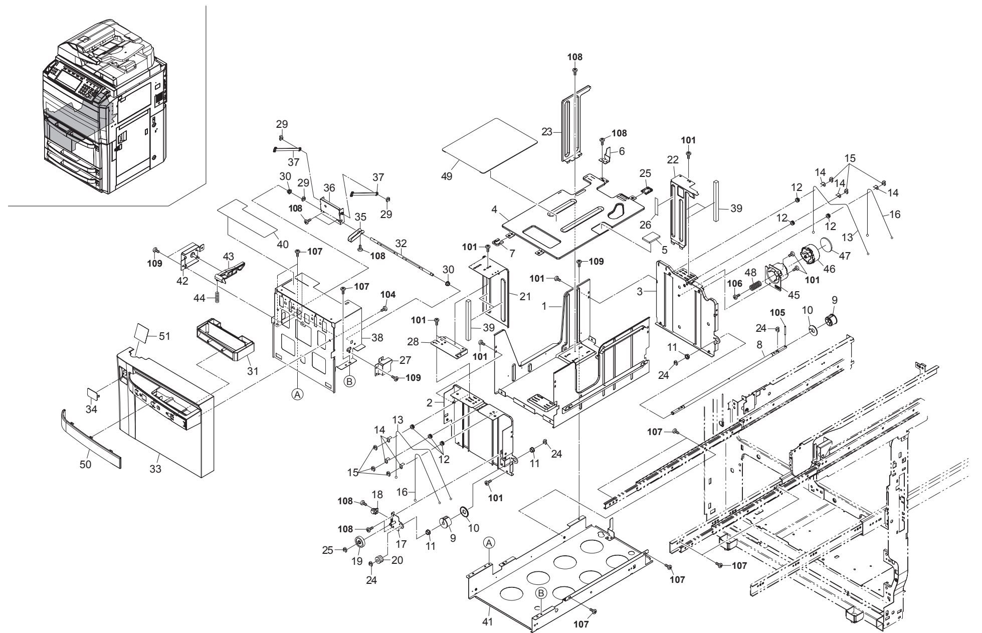
FIG. 6 Paper Deck 2
