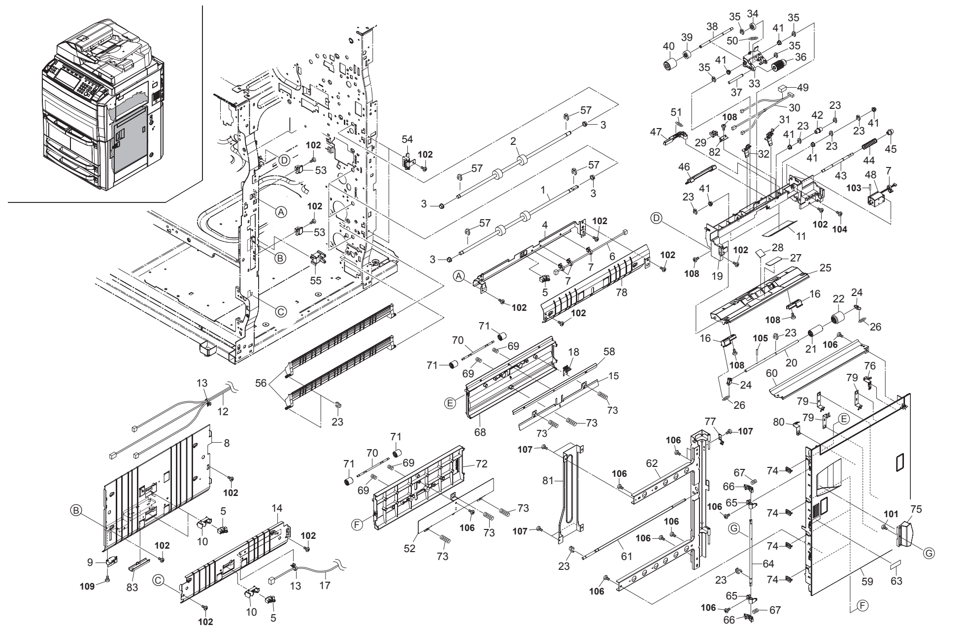
FIG. 9 Paper Feed Section 1
