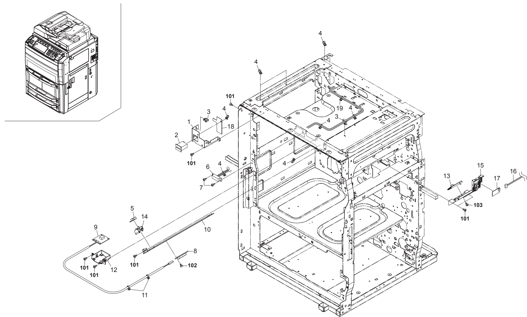
FIG. 32 Electrical Components 3
