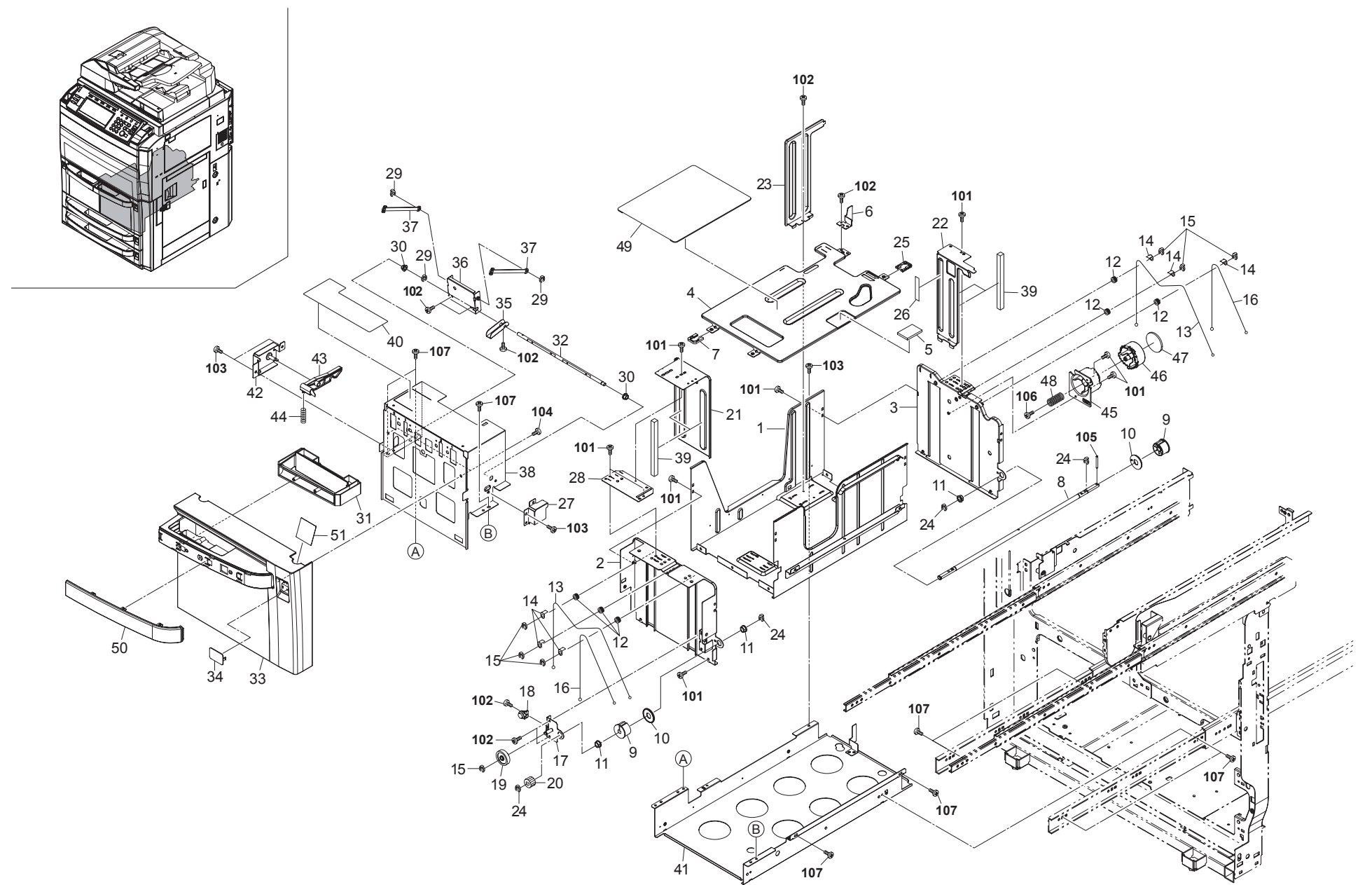
FIG. 5 Paper Deck 1
