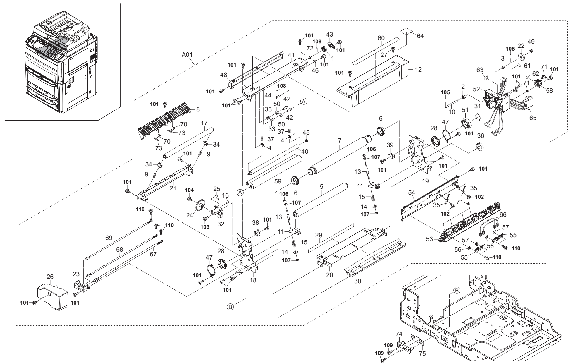
FIG. 21 Fuser Section 1
