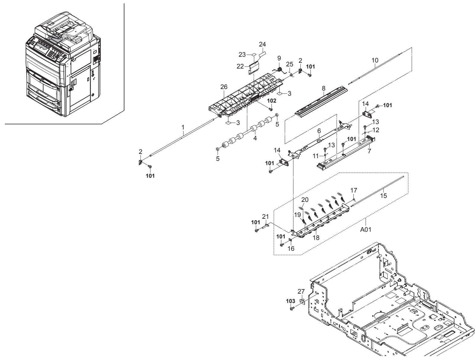
FIG. 22 Fuser Section 2
