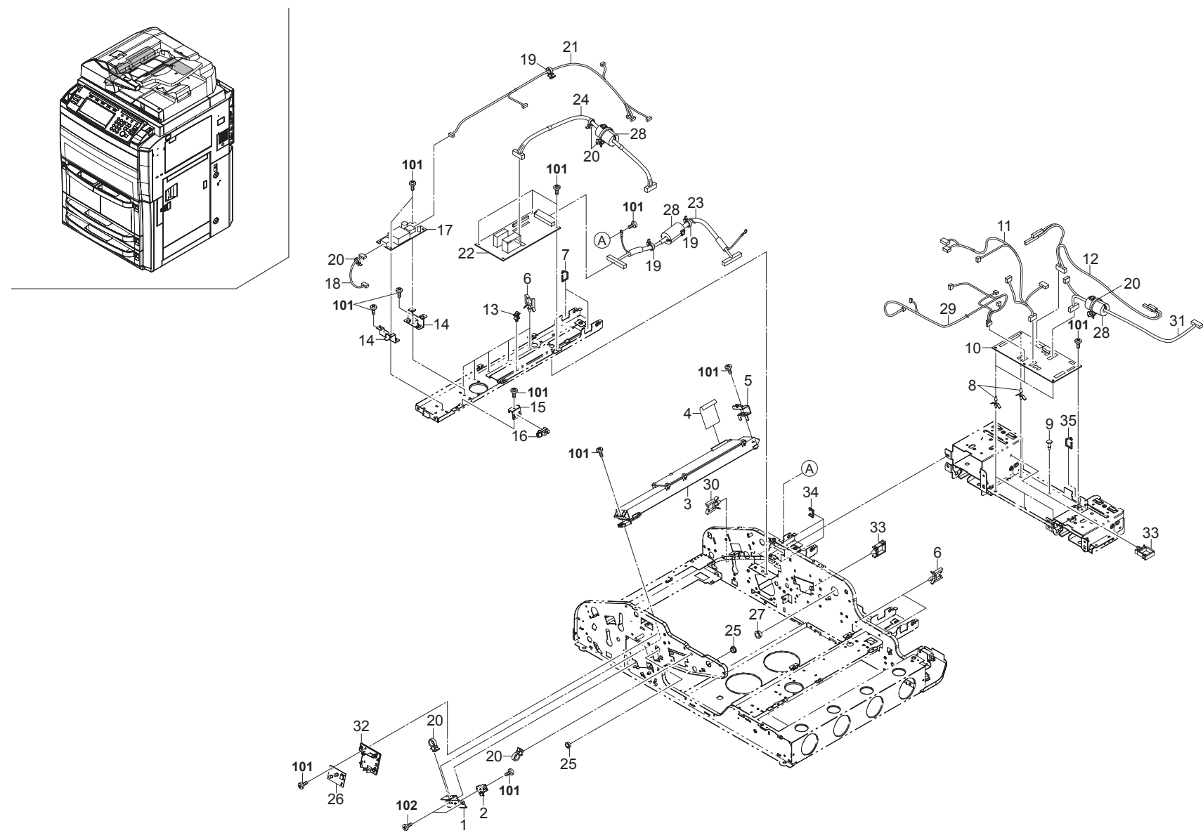
FIG. 41 Electrical Components (DP)
