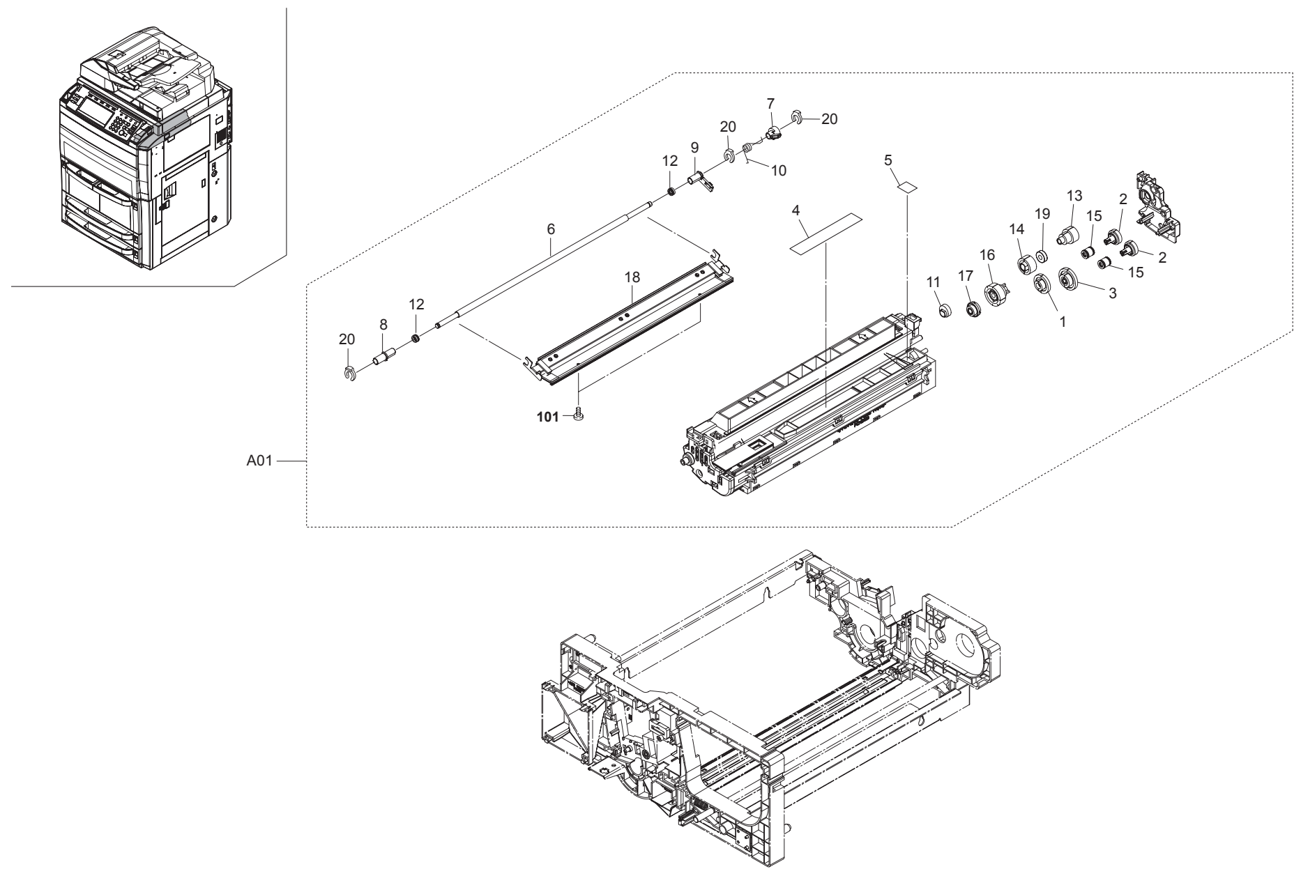
FIG. 18 Developing Section
