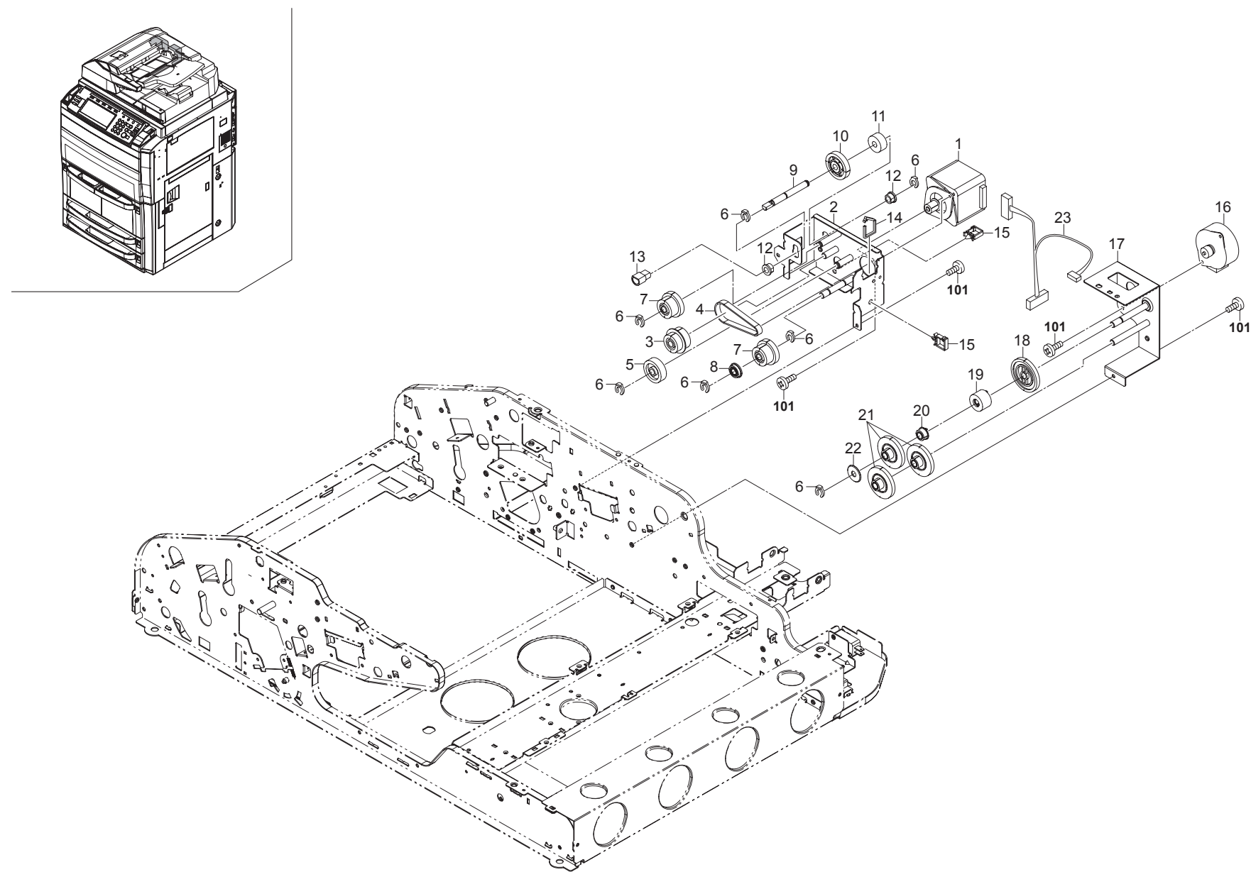
FIG. 40 Drive Section (DP)
