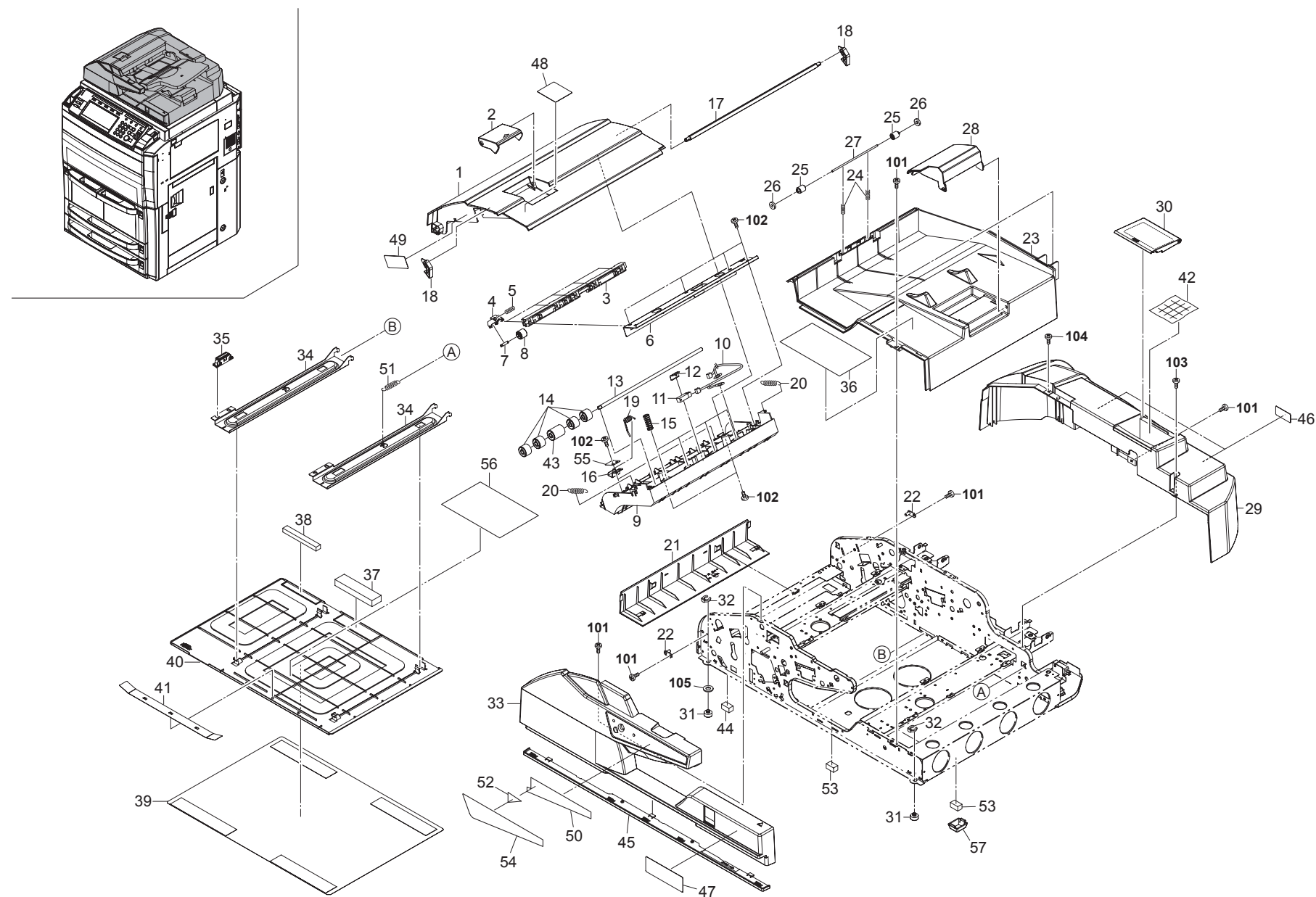
FIG. 34 Covers (DP)
