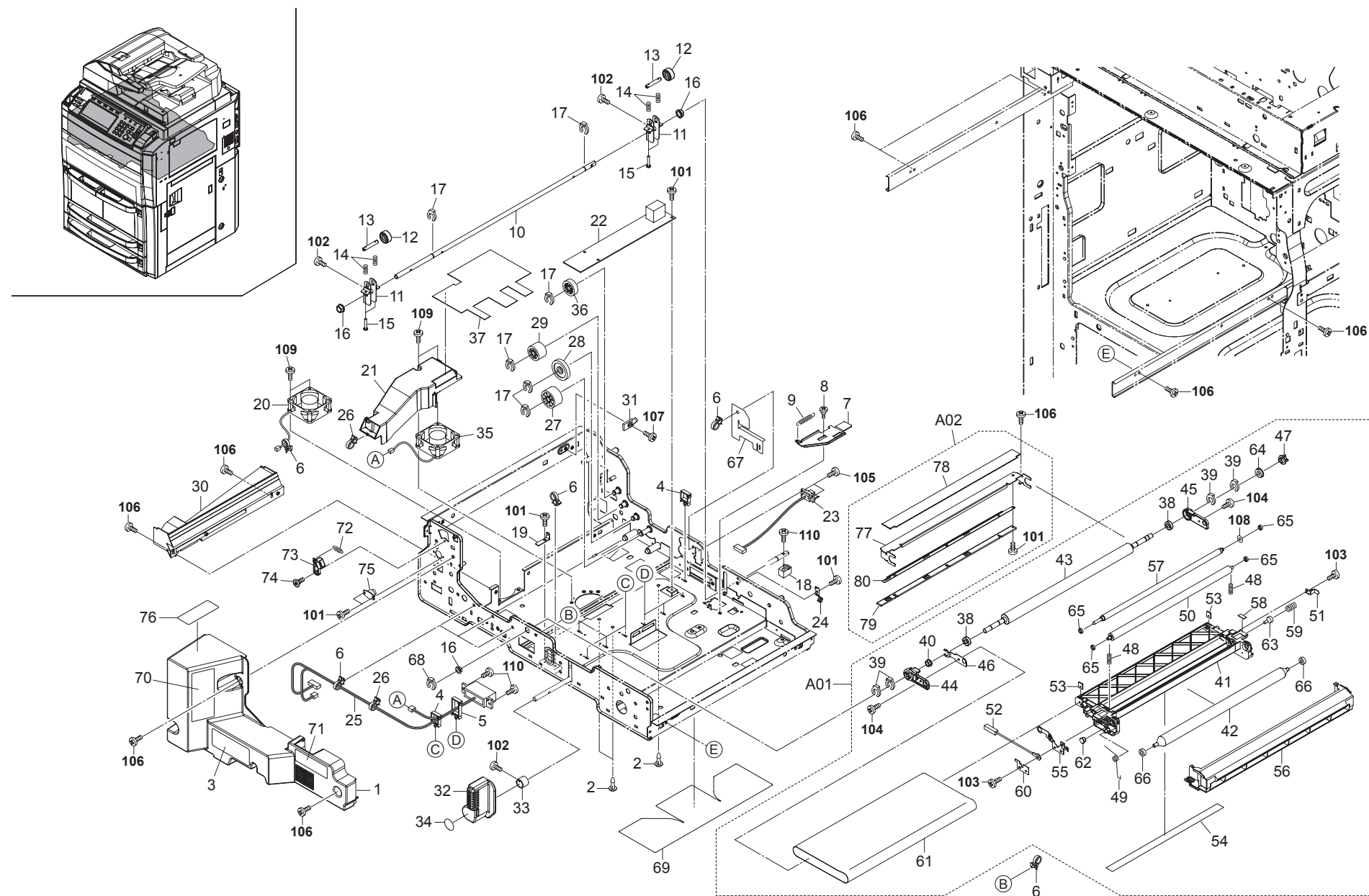
FIG. 12 Paper Conveying Section 1
