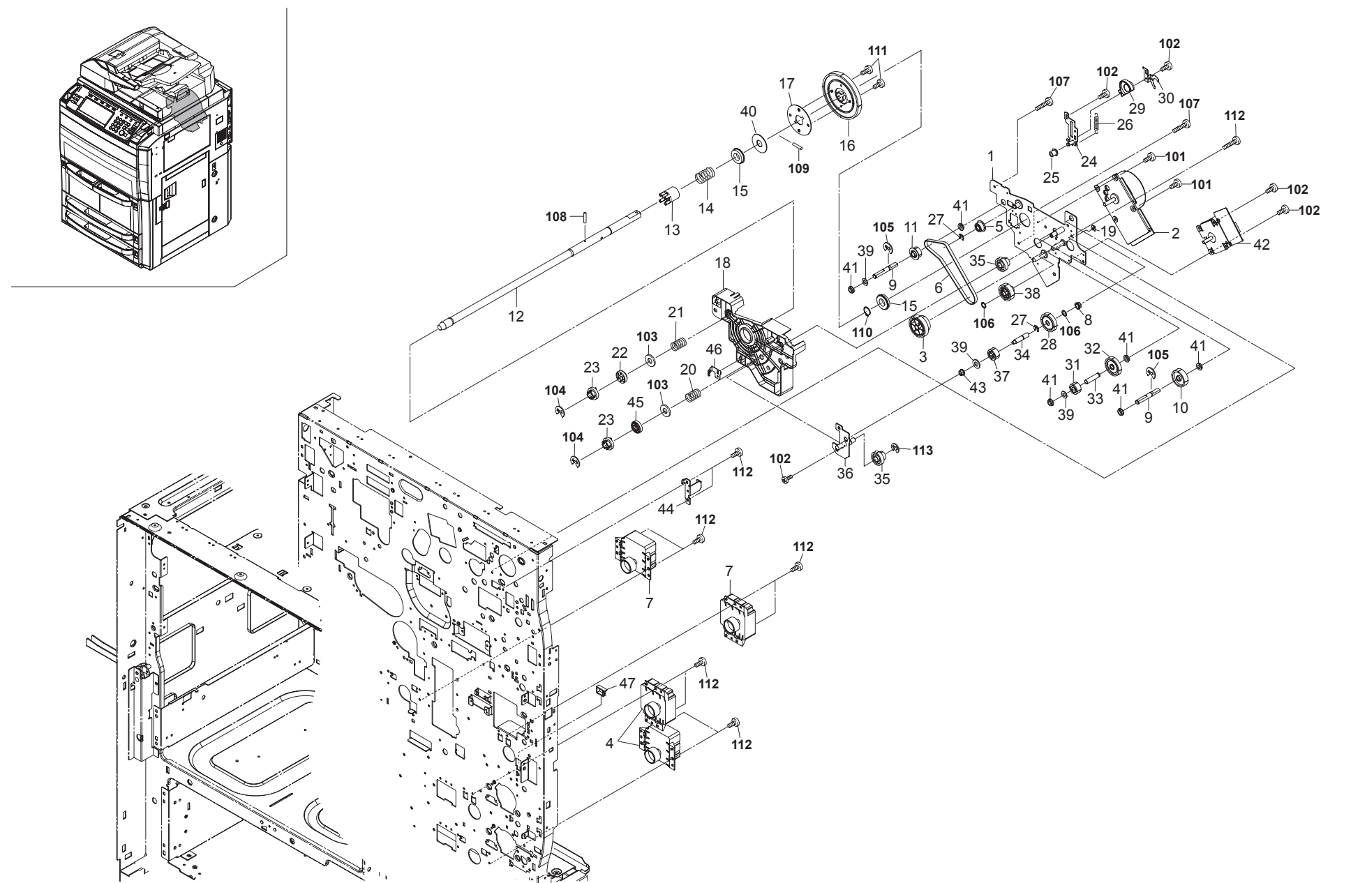
FIG. 24 Drive Section 2
