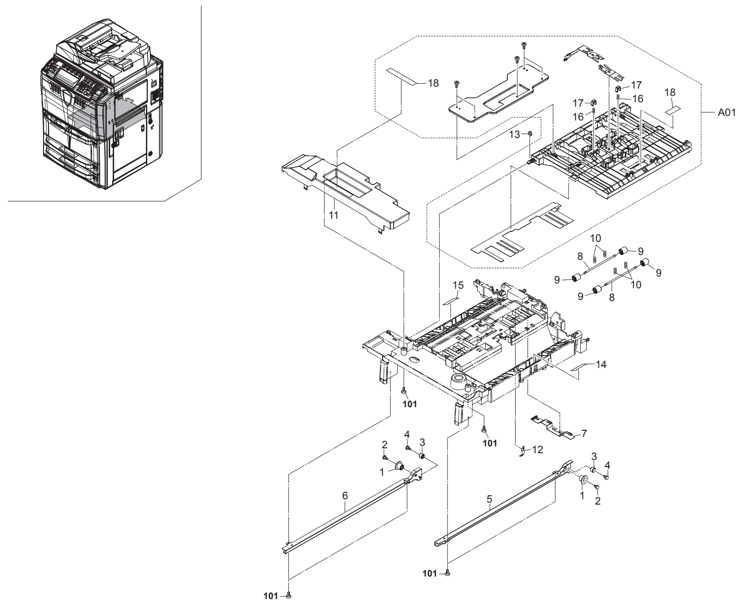
FIG. 8 Paper Deck Feed Section 2
