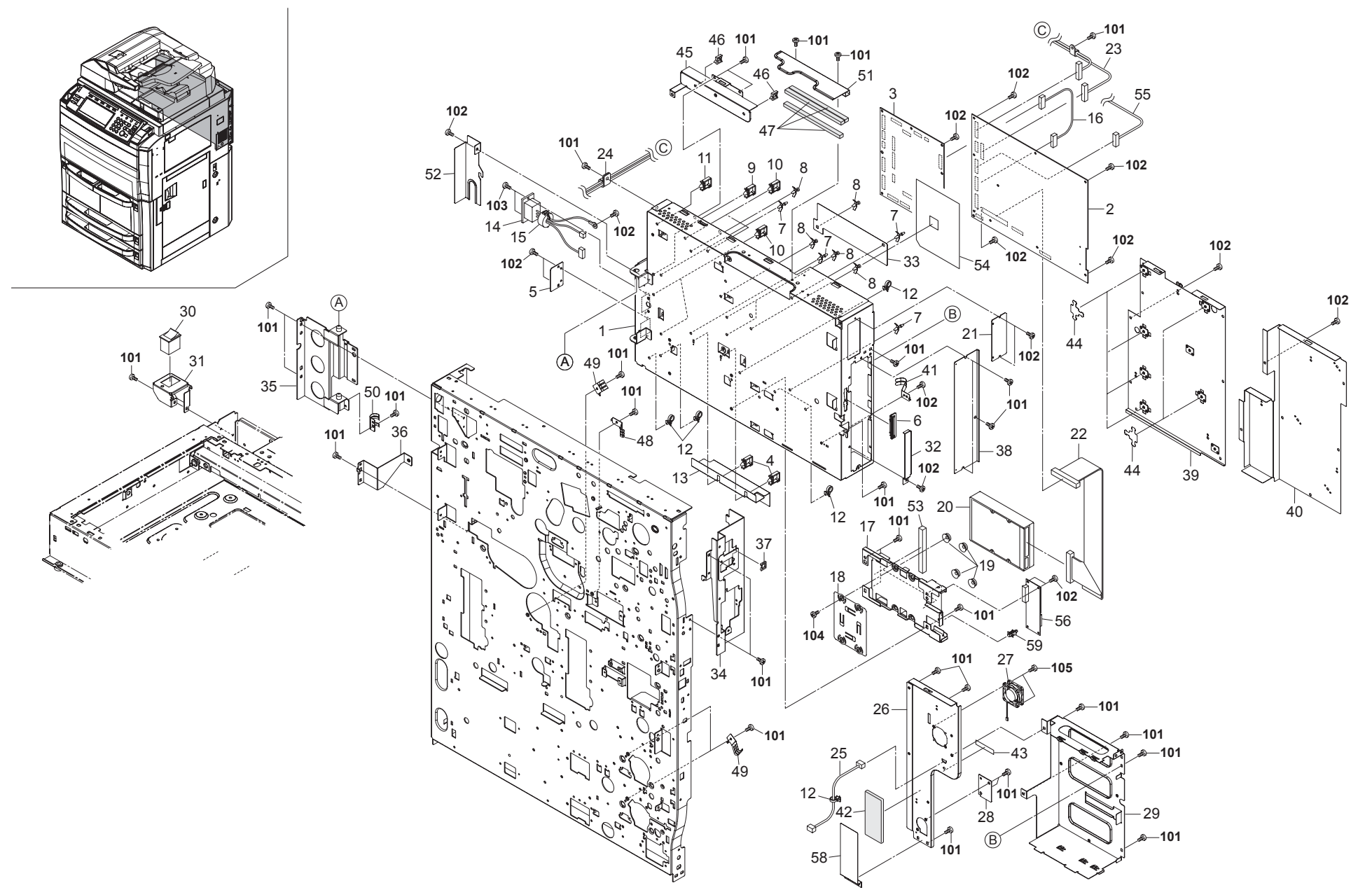
FIG. 31 Electrical Components 2
