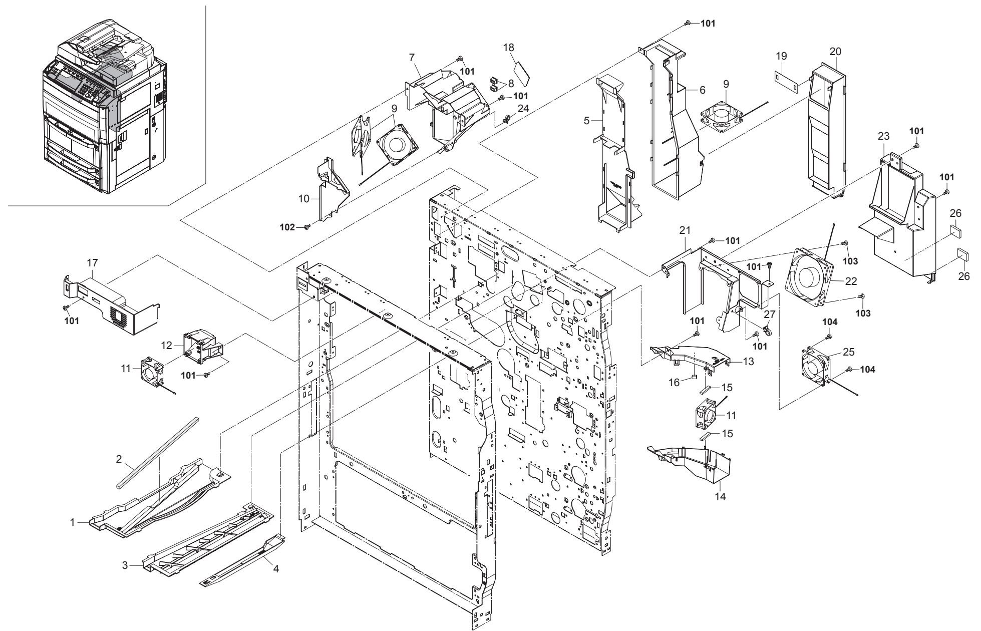
FIG. 25 Cooling Section
