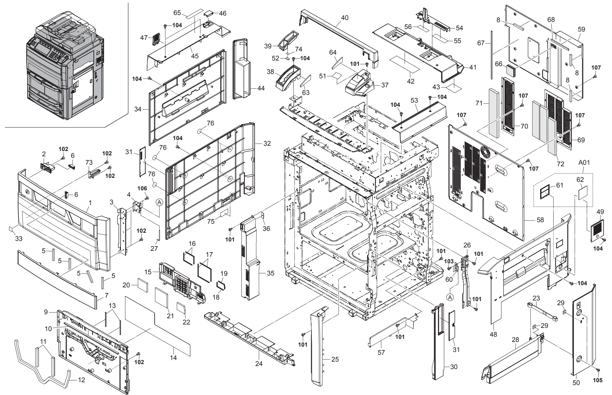
FIG. 1 Covers
