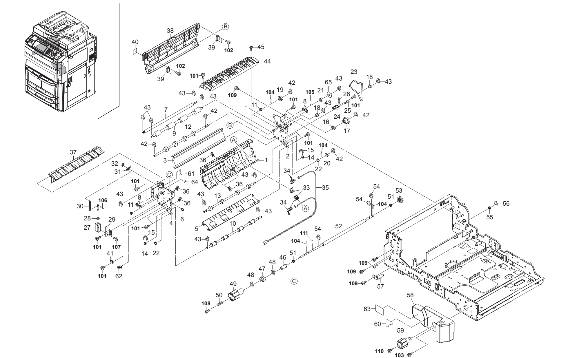
FIG. 14 Paper Conveying Section 3
