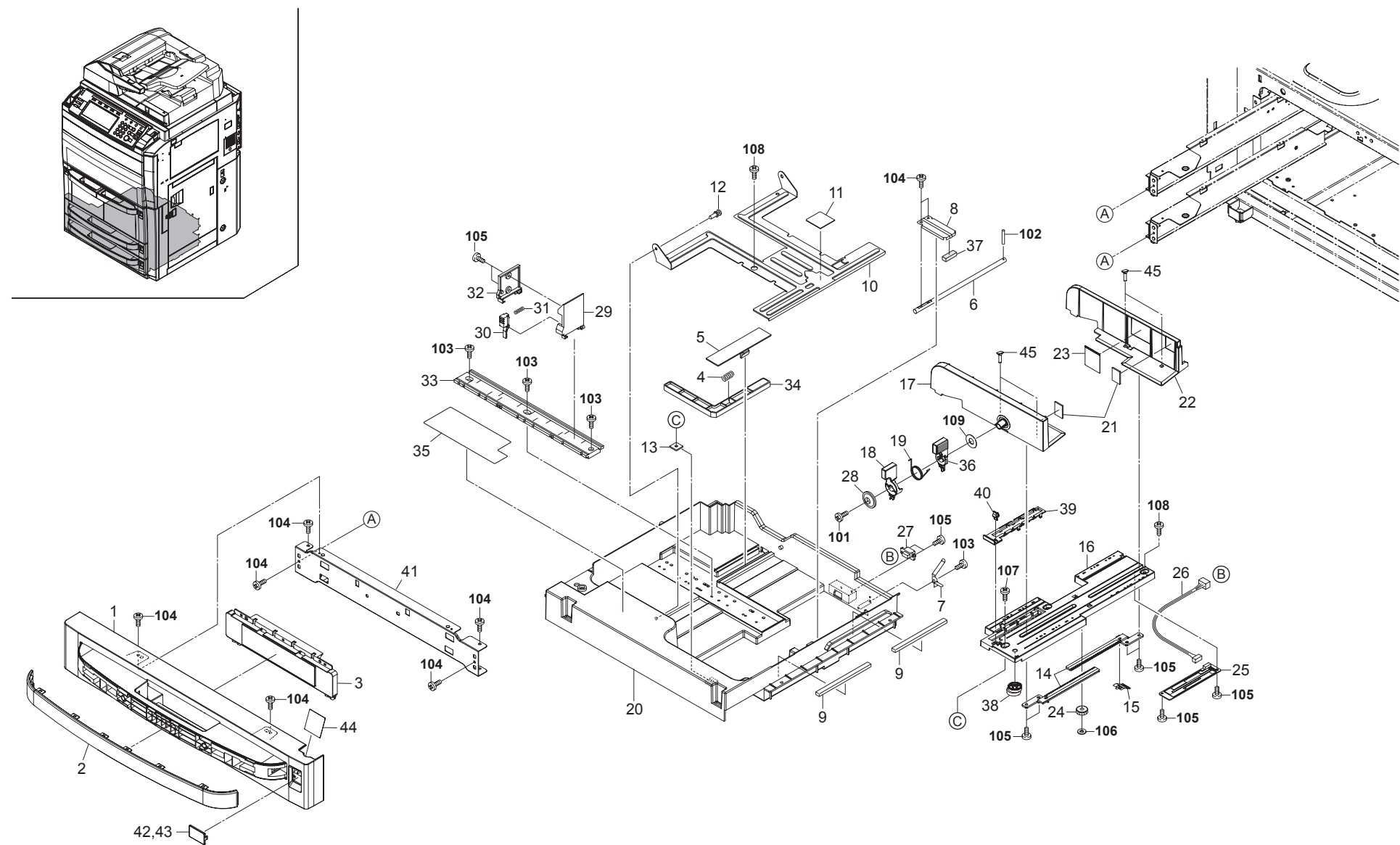
FIG. 4 Paper Cassette
