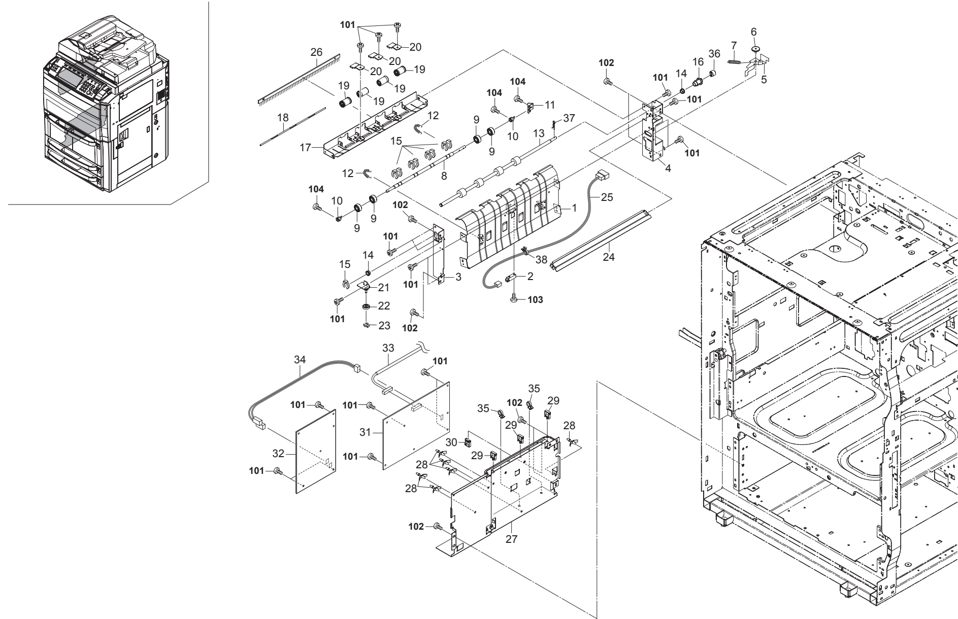
FIG. 29 Exit Section
