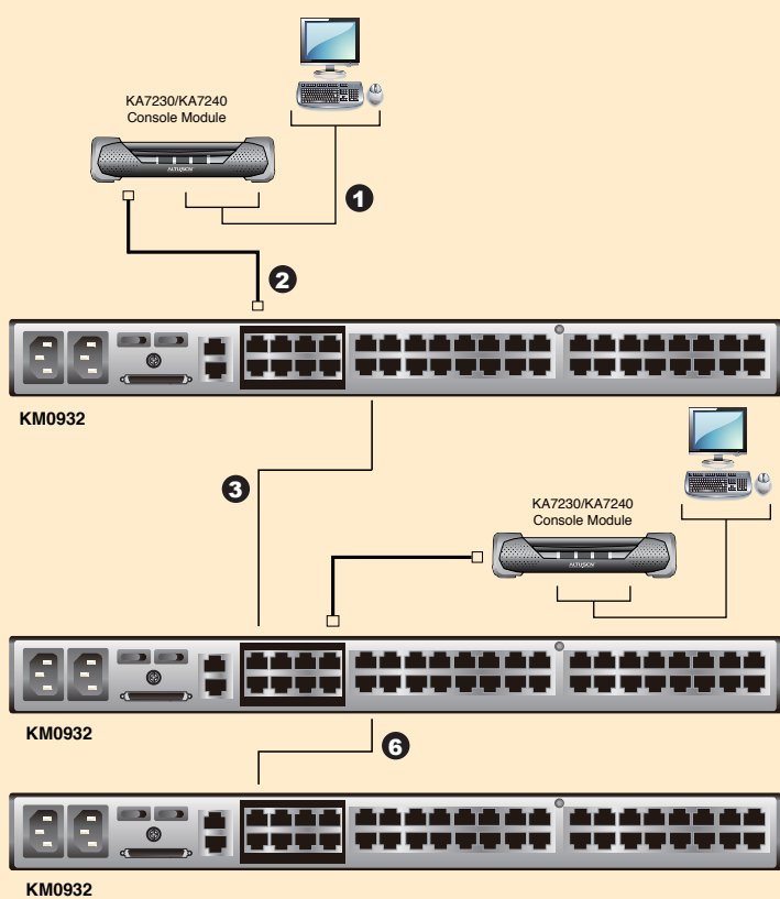
Cascaded KM0532 / KM0932 Installation Diagram
