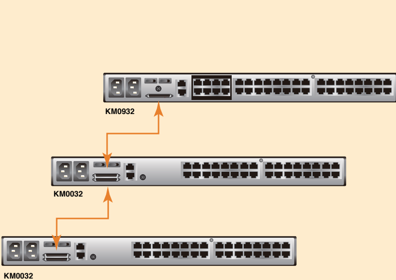
Daisy chained Installation Diagram
