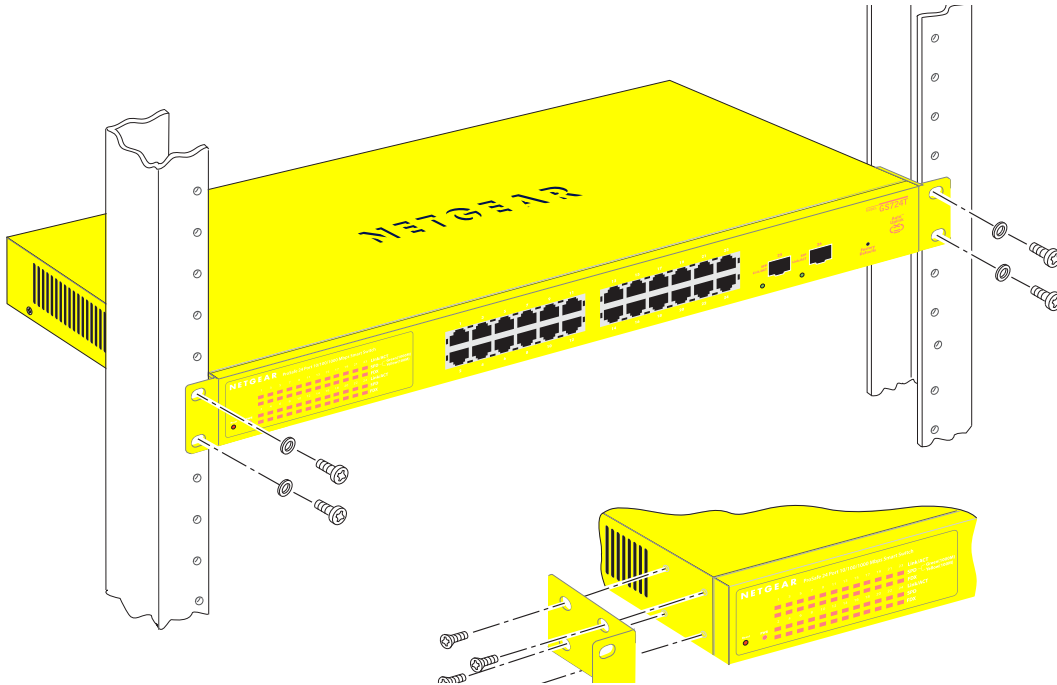
Figure 9. Rack Mount
