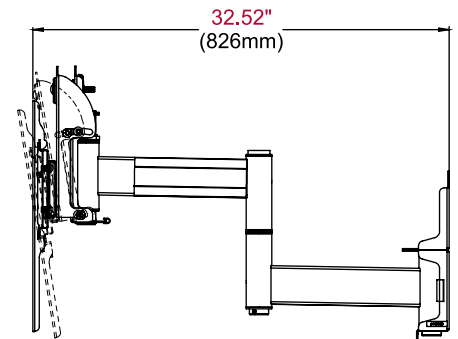
SIDE VIEW EXTENDED +10°/-5° TILT
