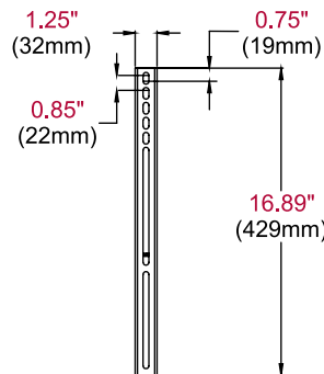
ADAPTOR BRACKET
