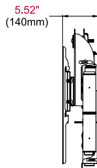
SIDE VIEW COLLAPSED
