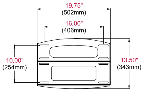
WALL PLATE
