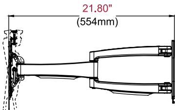
SIDE VIEW EXTENDED +15°/-5° TILT
