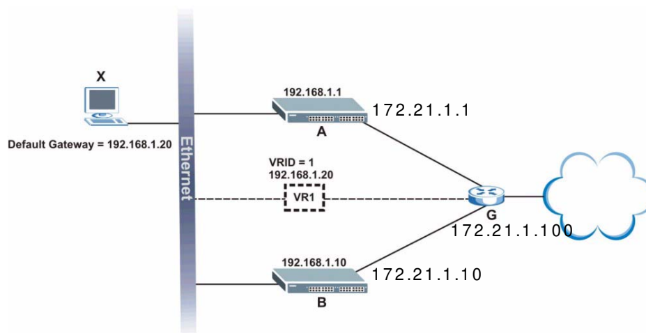
Figure 196 VRRP: Example 1
