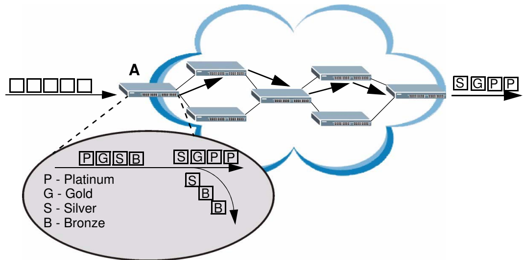
Figure 182 DiffServ Network
