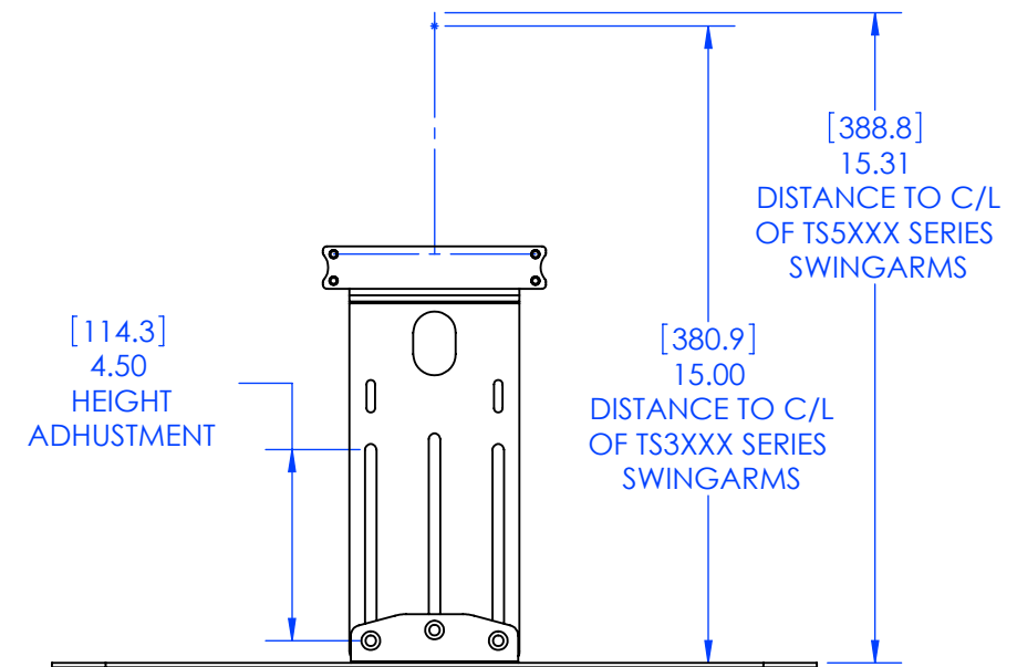
HIGHEST POSITION WITHOUT EXTENDER BRACKET
