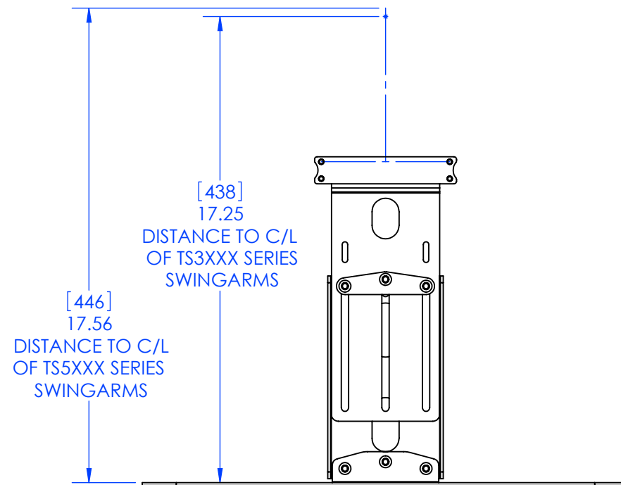
HIGHEST POSITION WITH EXTENDER BRACKET
