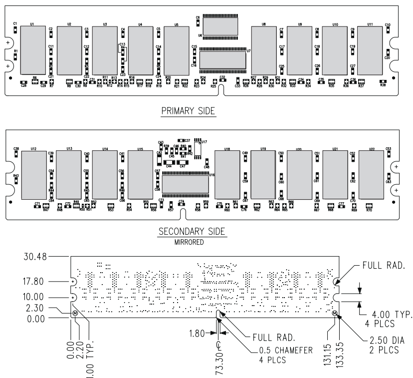
Figure 1: KVR400X72RC3AK2/1G 184-Pin DIMM Kit
