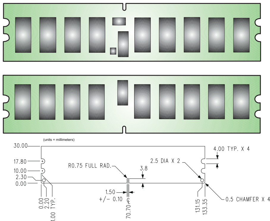
Figure 1: KVR667D2S4P5/2GEF 240-Pin DIMM
