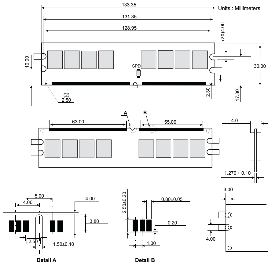
Figure 1: KVR667D2/1GR 240-Pin DIMM
