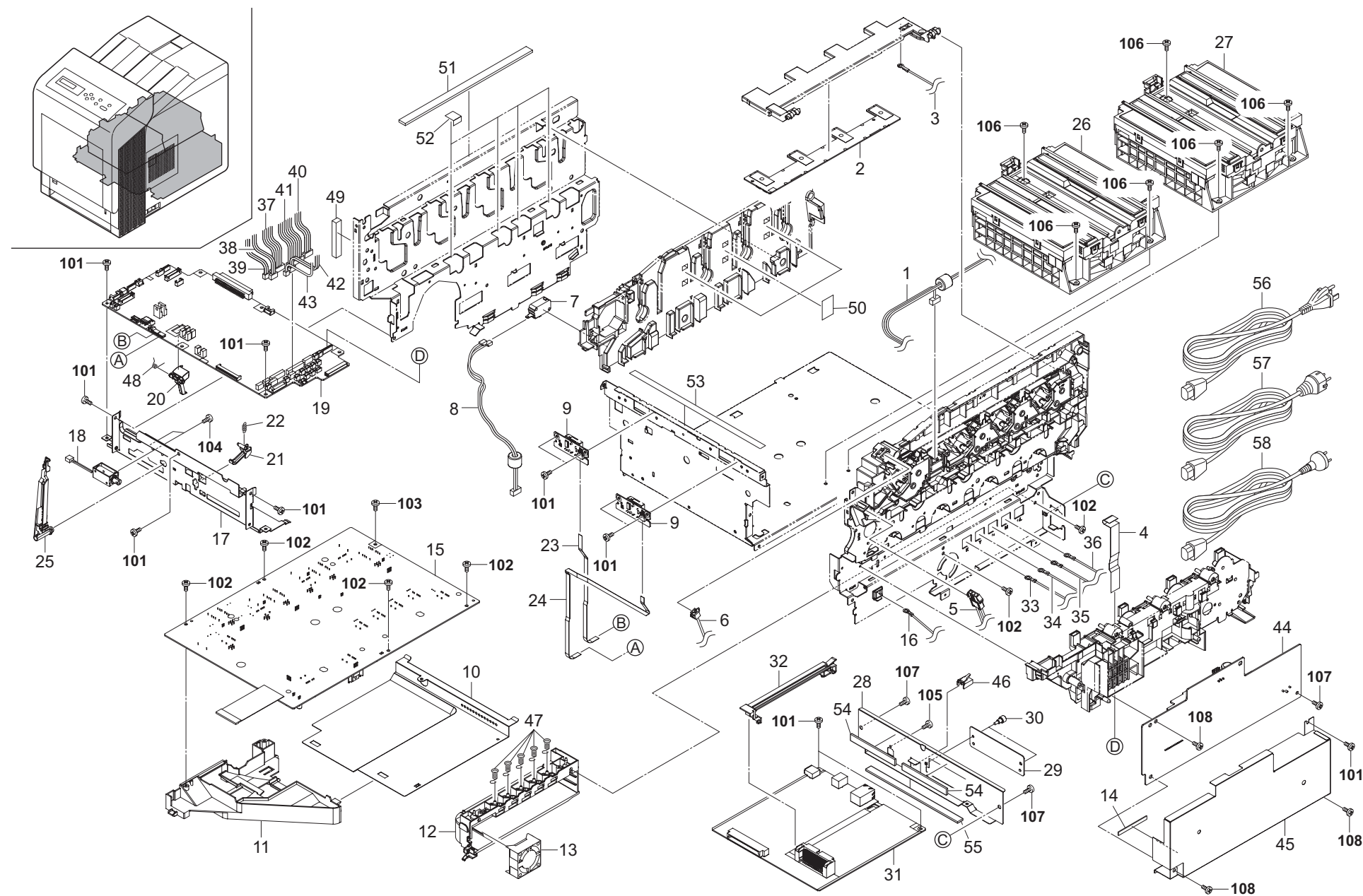
FIG. 14 Electrical Components
