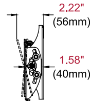
SIDE VIEW VESA 75/100 +15°/-5° TILT
