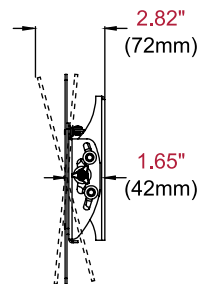
SIDE VIEW VESA 100/200 +15°/-5° TILT
