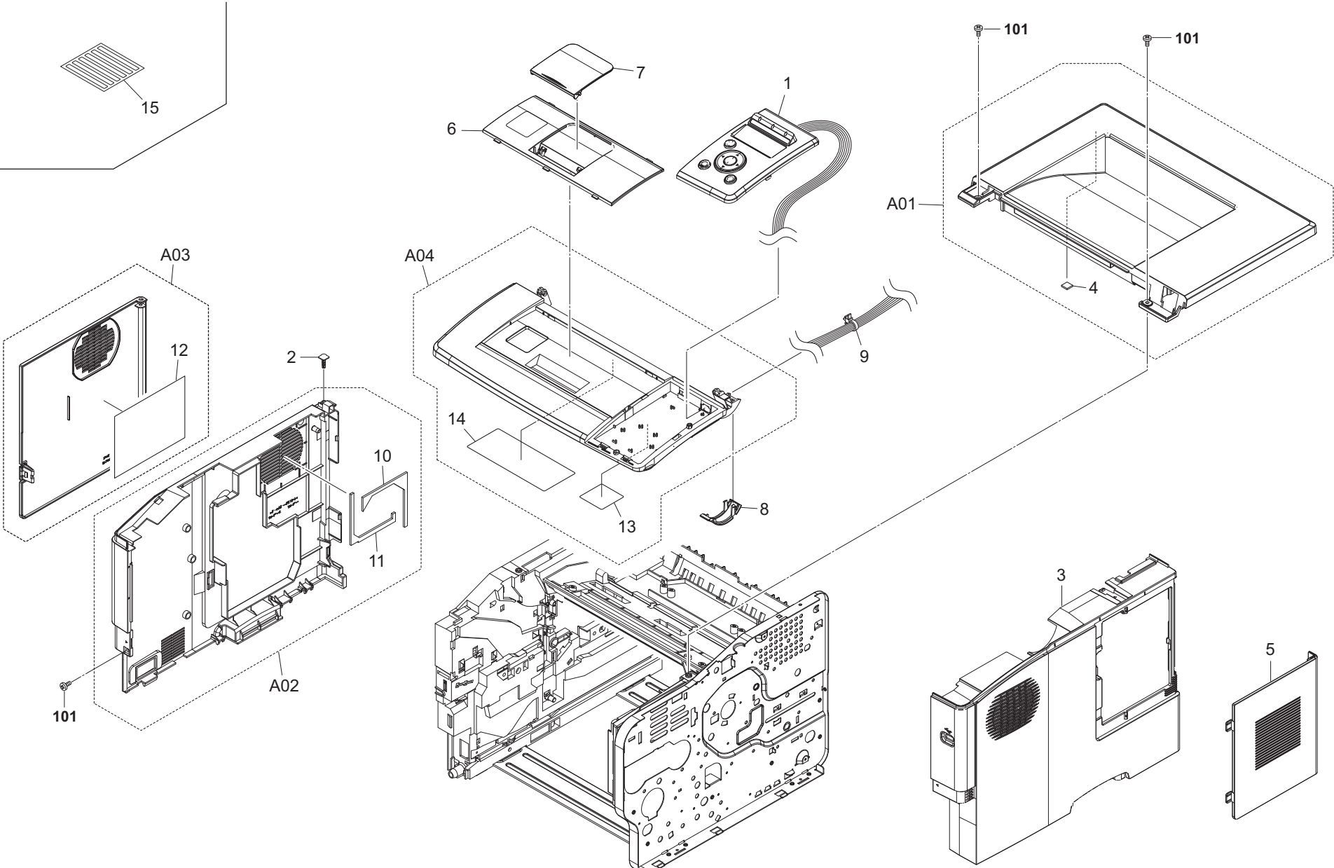
FIG. 1 Covers (FS-2020D)
