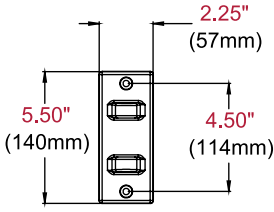
WALL PLATE DETAIL
