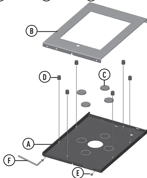
PTS 11XX Secure Tablet Enclosure
