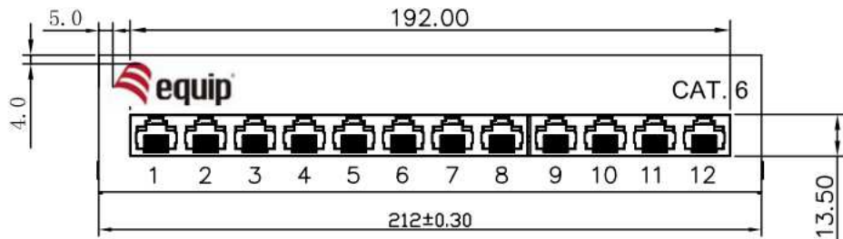
Plan View
