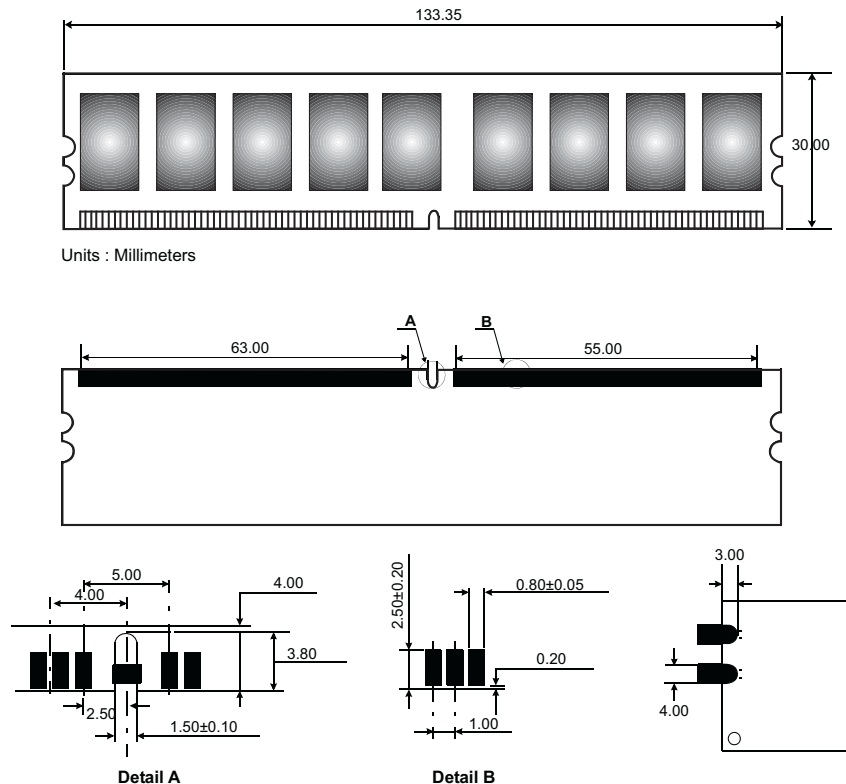
Figure 1: KVR800D2E6K2/1G 240-Pin DIMM
