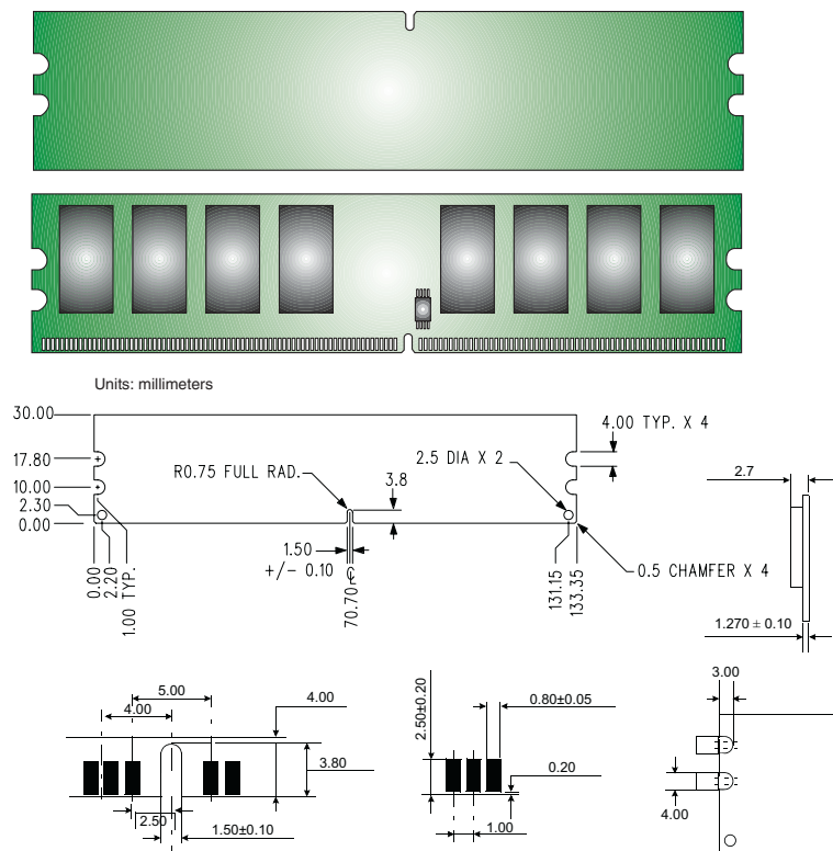
Figure 1: KVR1066D2N7K2/1G 240-Pin DIMM
