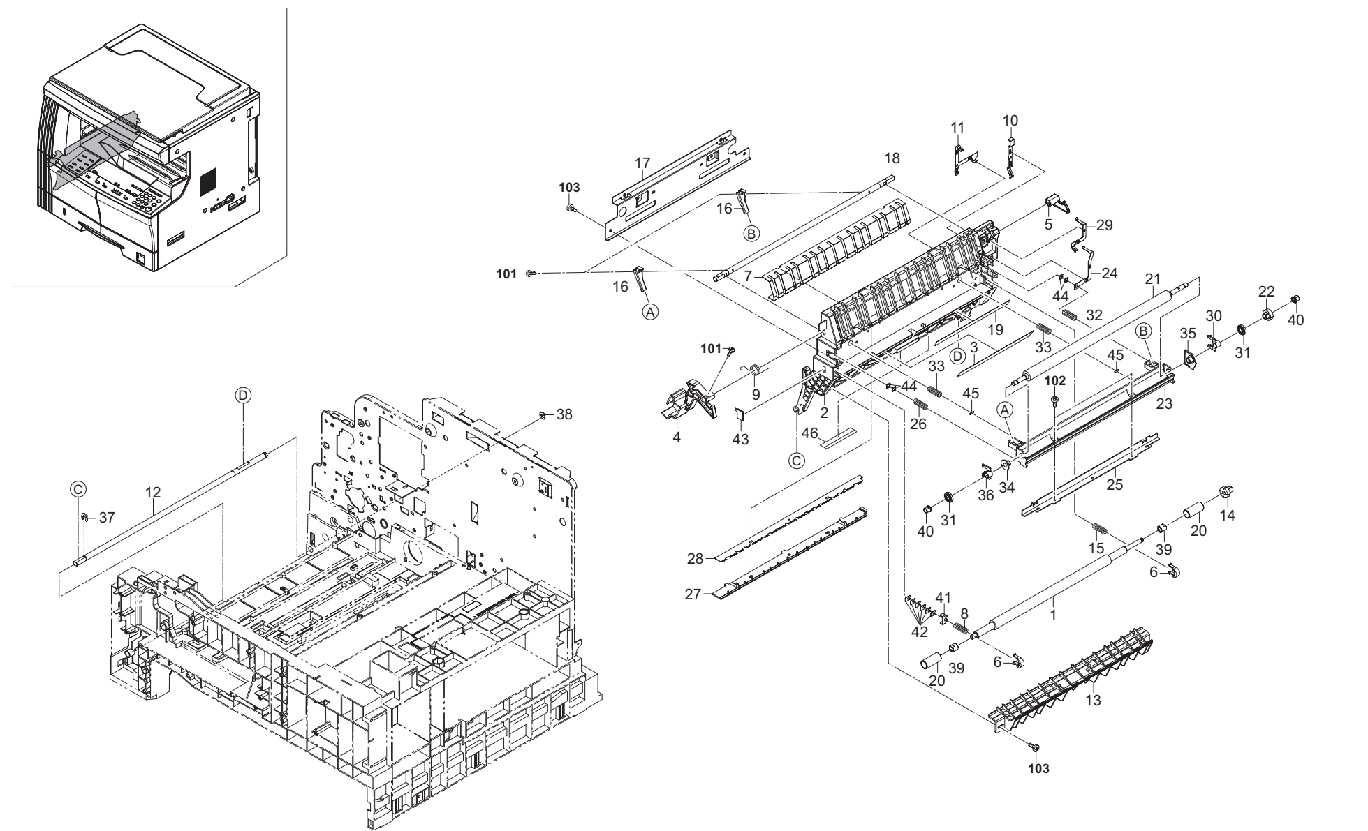
FIG. 4 Conveying Section
