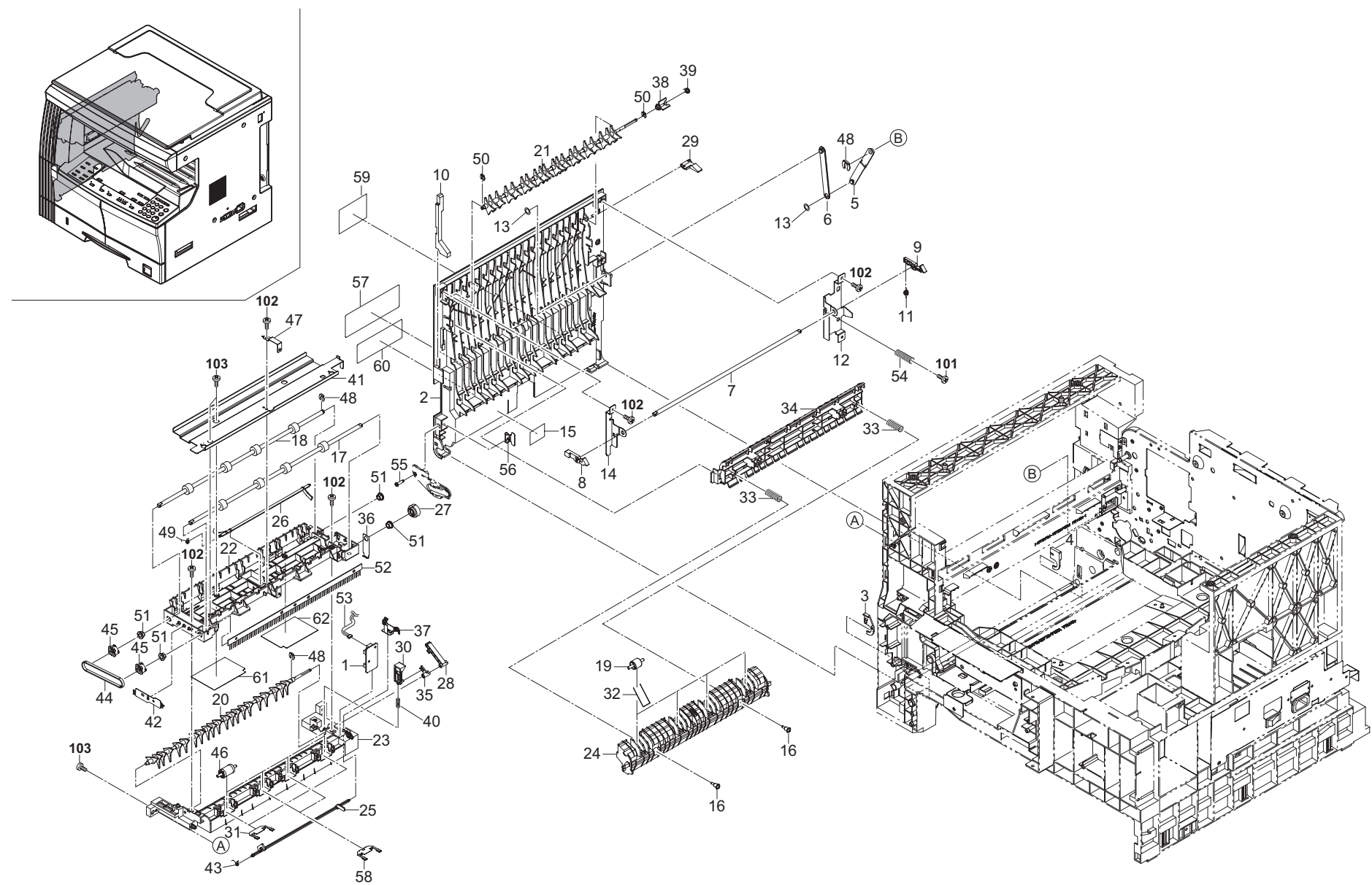
FIG. 7 Exit Section
