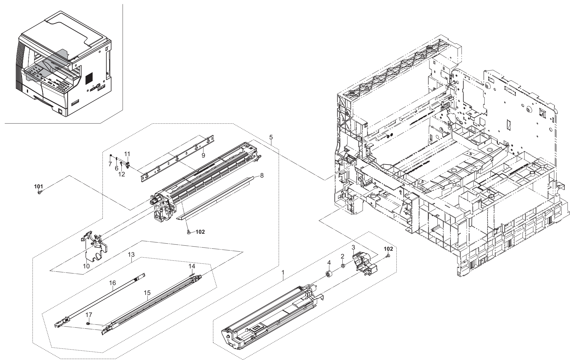
FIG. 9 Imaging Unit
