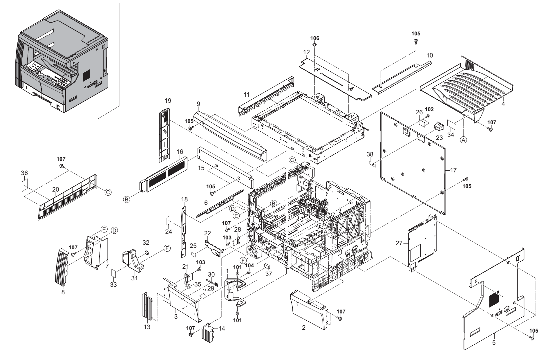
FIG. 1 Exterior Covers
