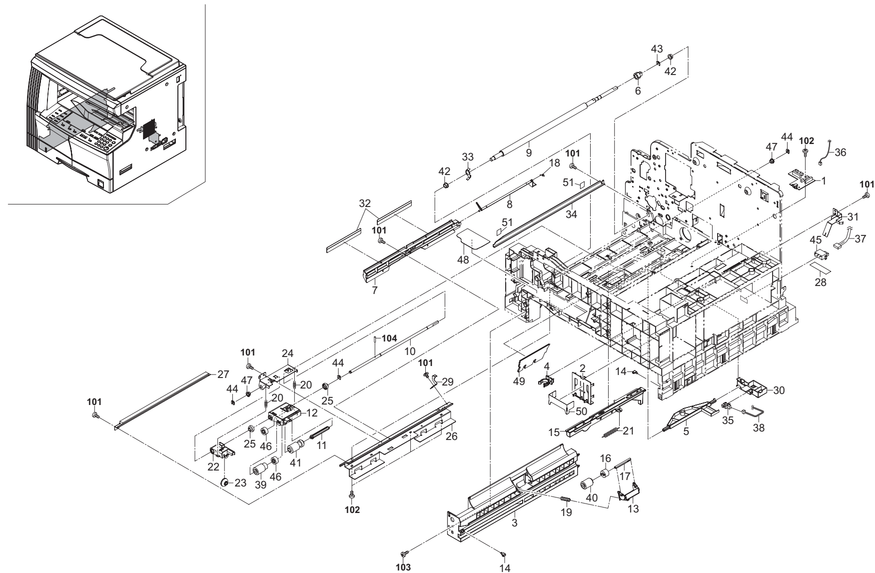
FIG. 5 Paper Feed Section
