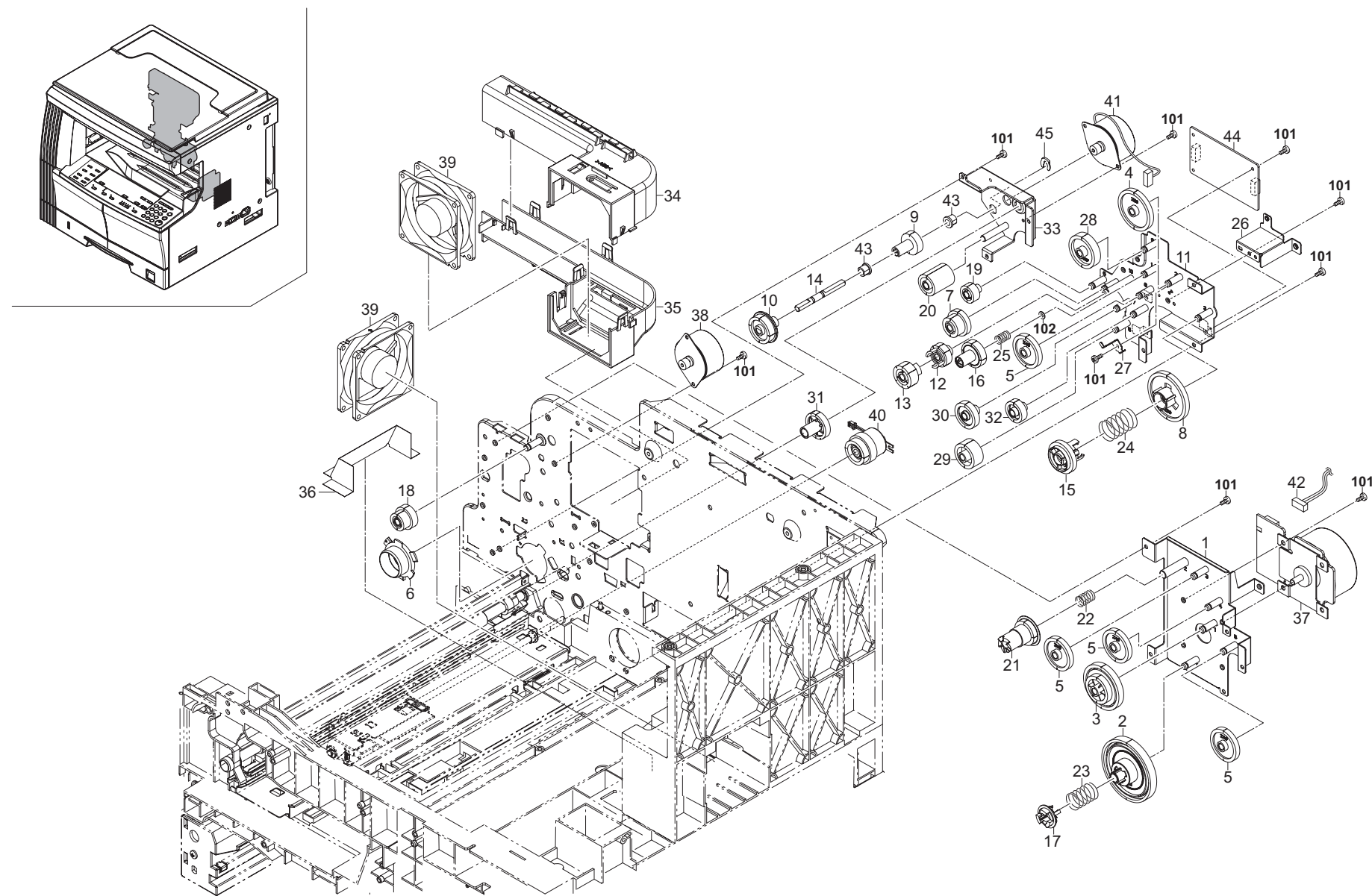
FIG. 11 Driving & Cooling Section
