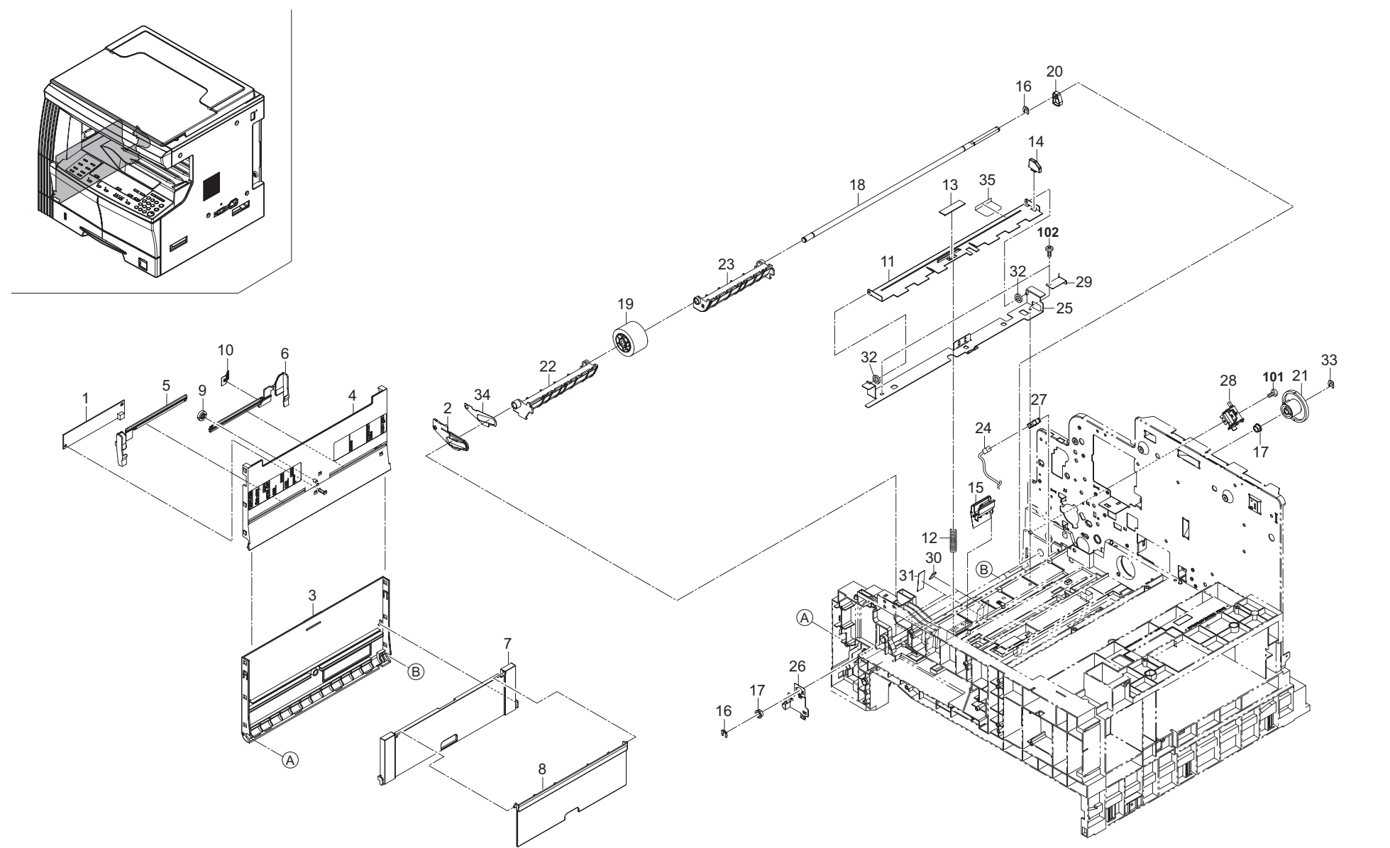
FIG. 6 Bypass Section
