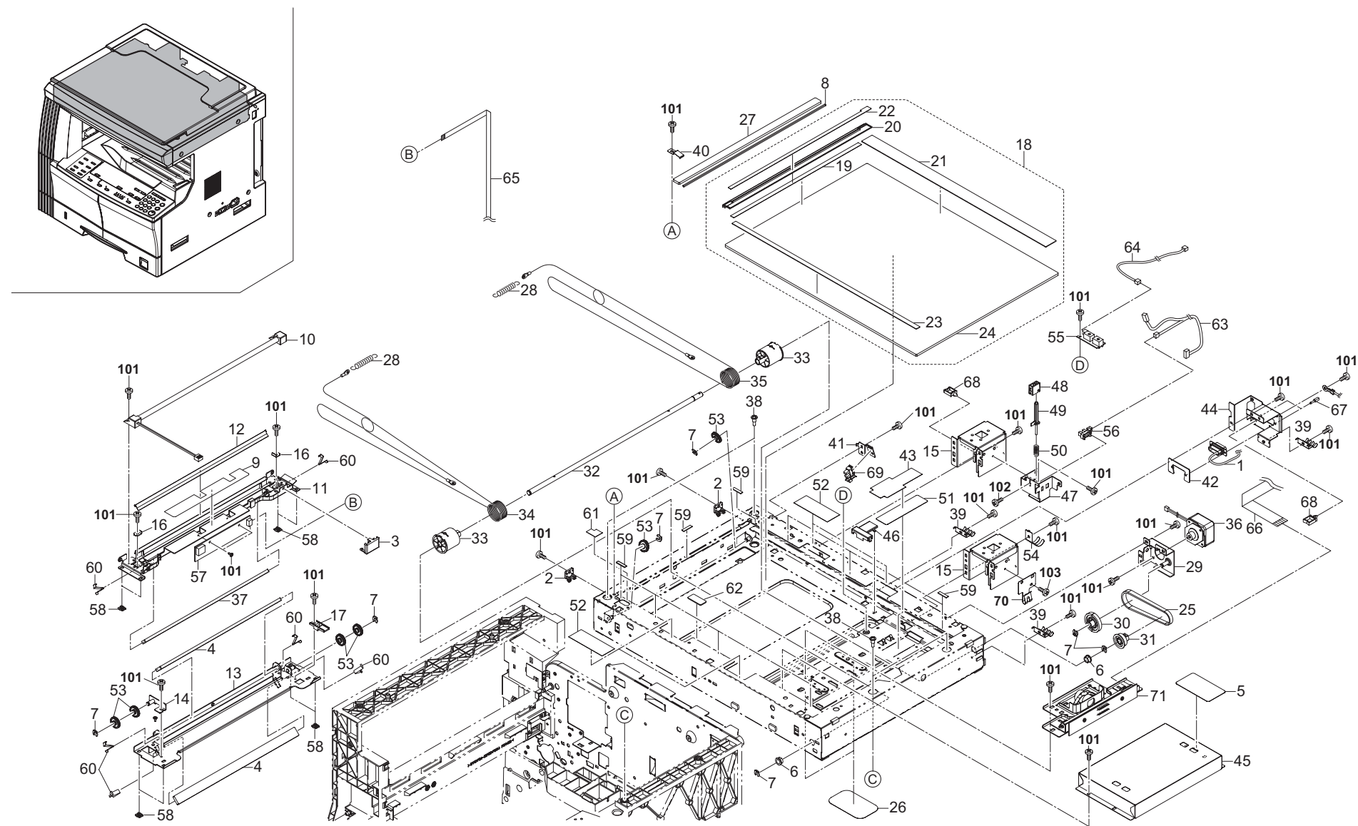
FIG. 8 Scanner Section
