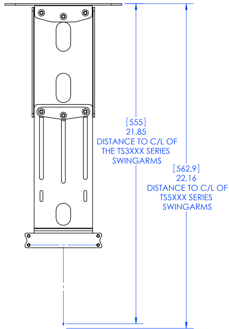
HIGHEST EXTENSION
