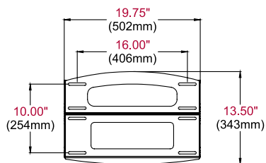
WALL PLATE
