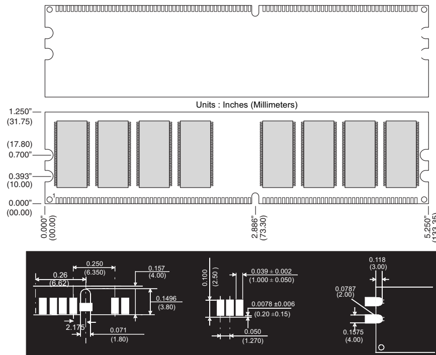
Figure 1: KVR400/256R 184-Pin DIMM
