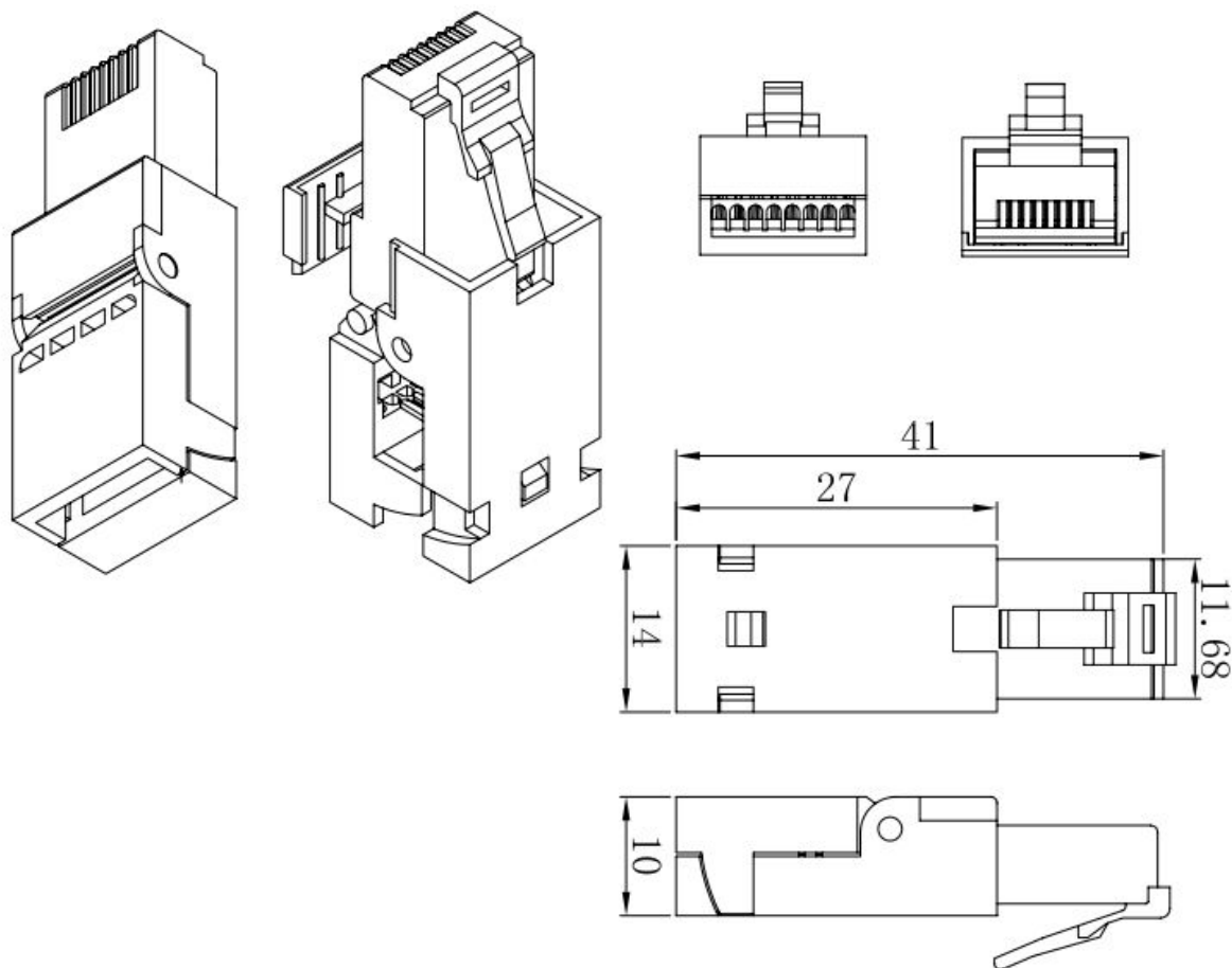
TIA/EIA-568 T568A termination
