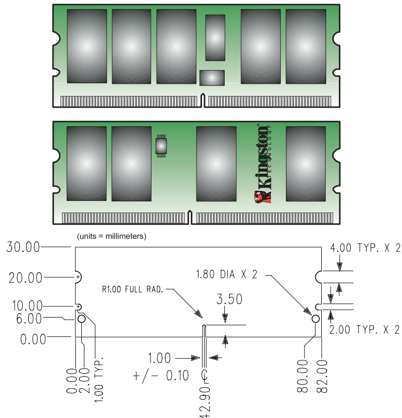
Figure 1: KVR400D2M3/512 244-Pin MiniDIMM
