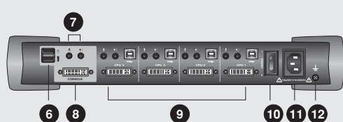
CS1184 Rear View
