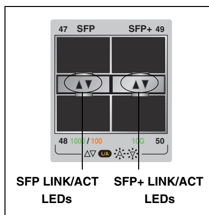
Figure 19. SFP and SFP+ LEDs on x610-48Ts/X and x610-48Ts/X-POE+ Switches
