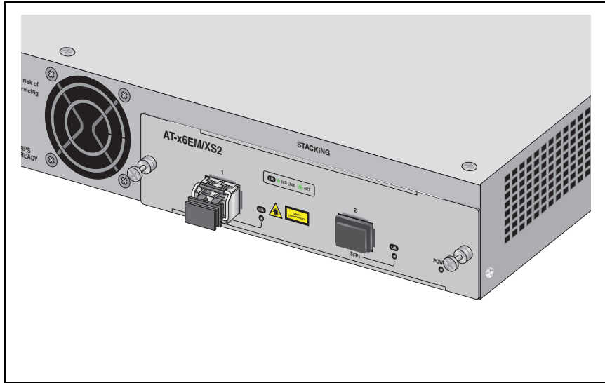
Figure 66. Positioning the SFP+ Transceiver Locking Handle
