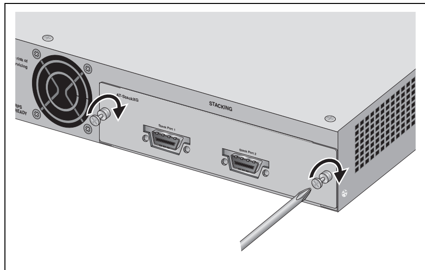
Figure 61. Securing the AT-StackXG Stacking Module
