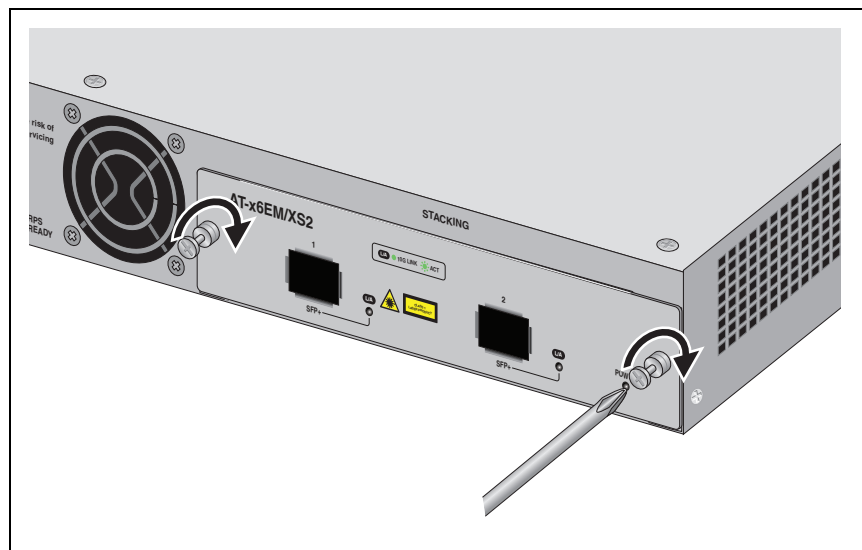
Figure 62. Securing the AT-x6EM/XS2 Stacking Module
