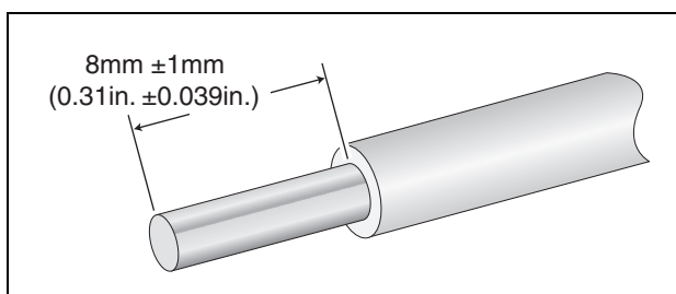
Figure 72. Stripped Wire
