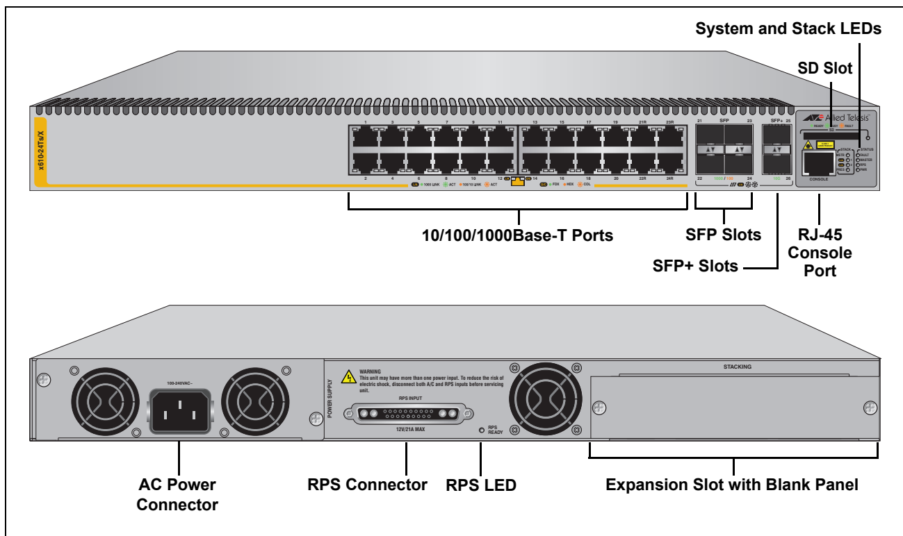
Figure 2. x610-24Ts/X Switch
