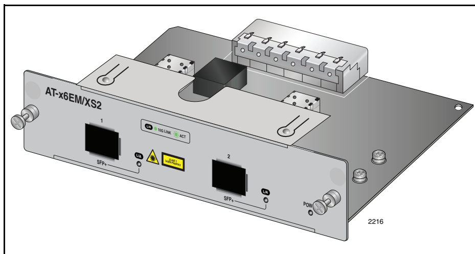
Figure 57. AT-x6EM/XS2 Stacking Module
