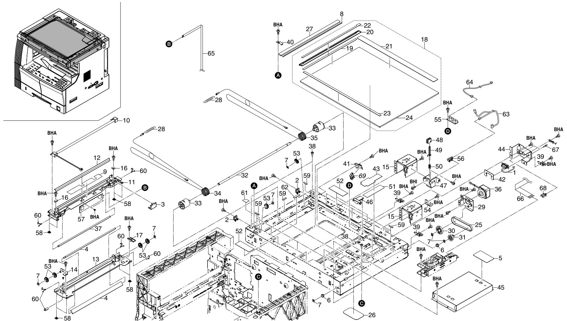
FIG. 8 SCANNER SECTION
