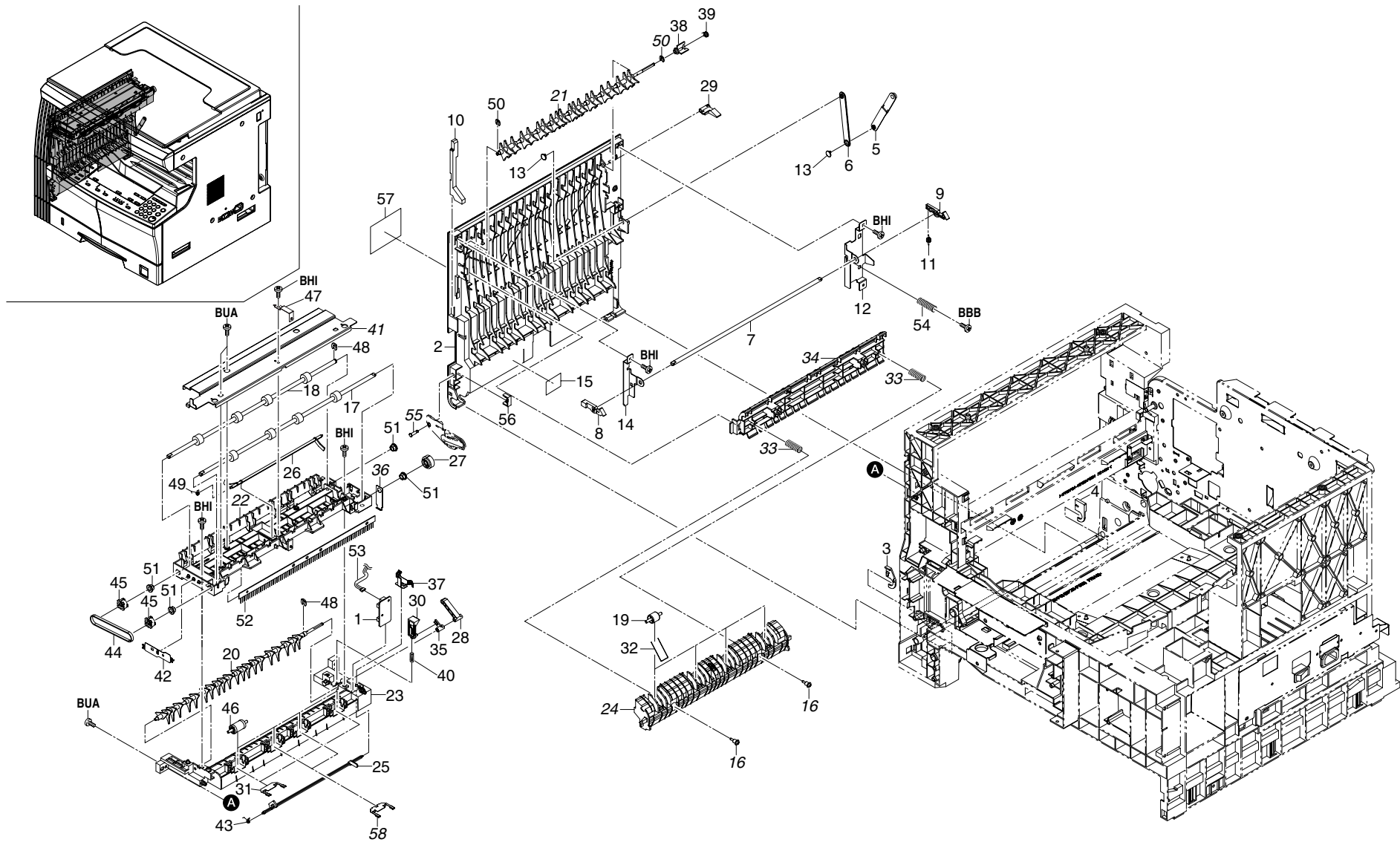
FIG. 7 EXIT SECTION
