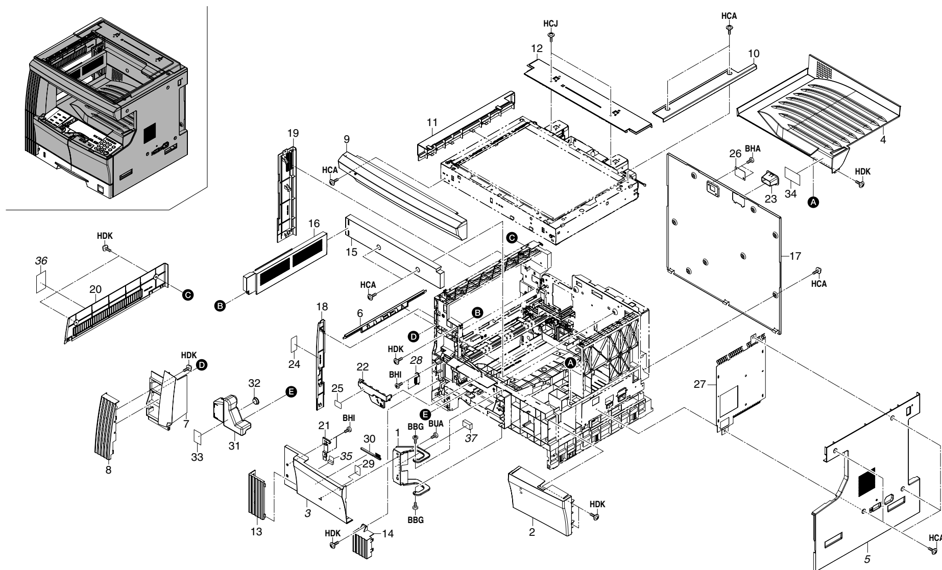
FIG. 1 EXTERIOR COVERS
