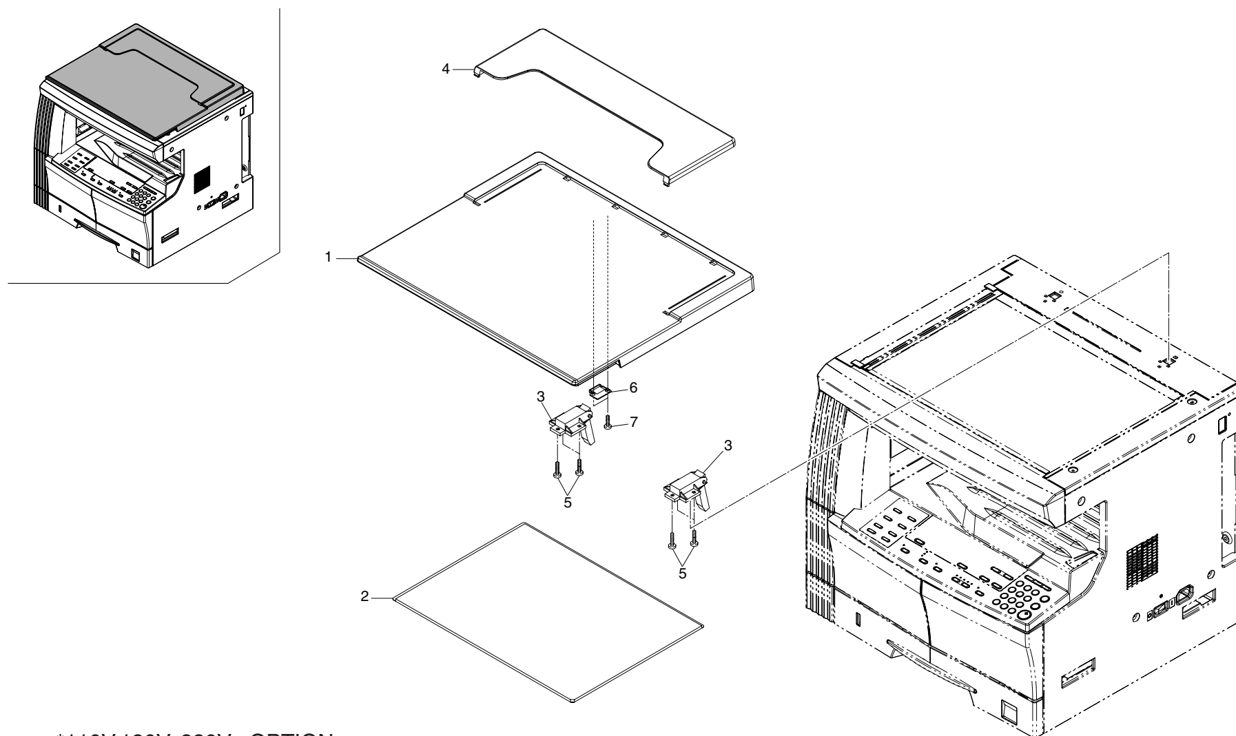
FIG. 14 ORIGINAL HOLDER
