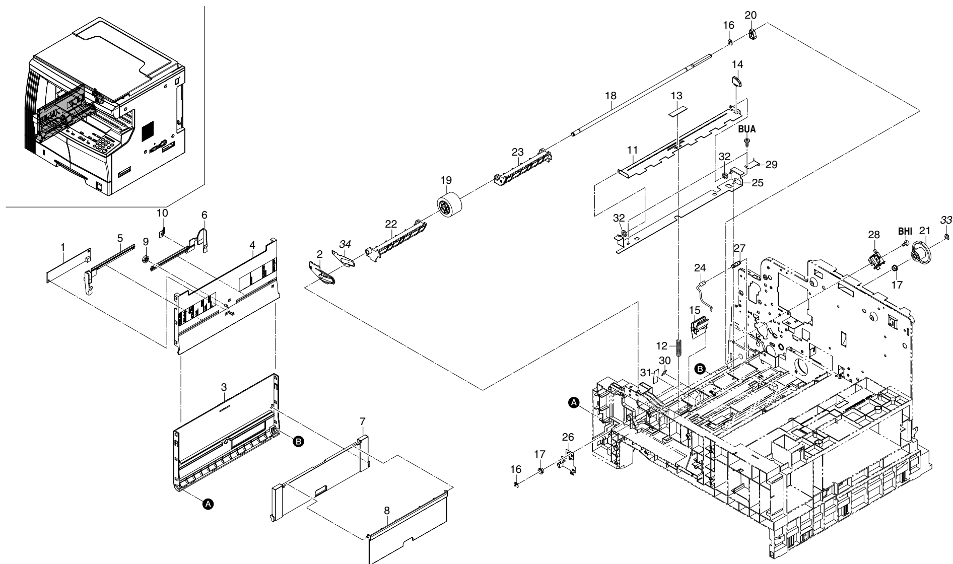
FIG. 6 BYPASS SECTION
