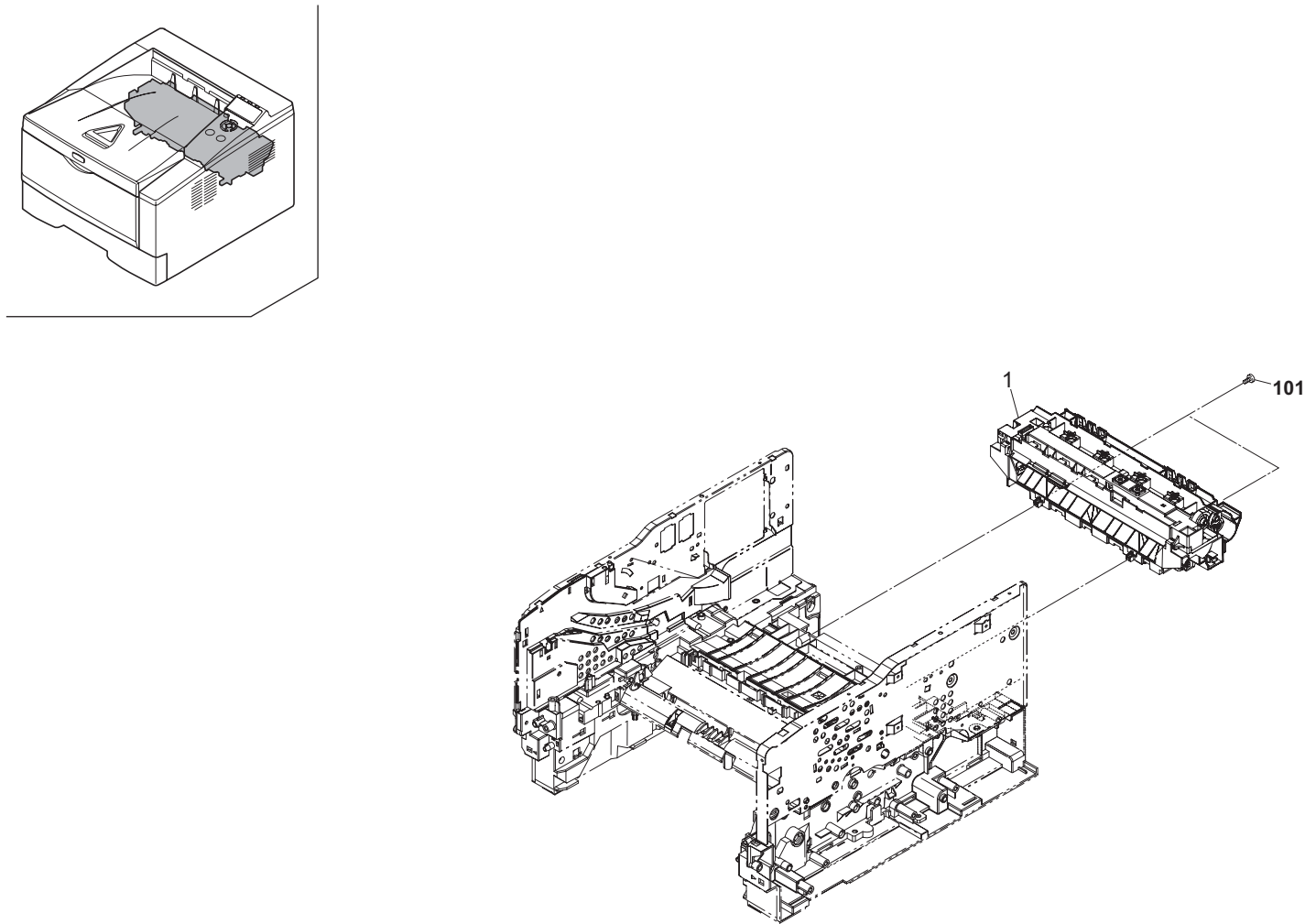
FIG. 8 Fuser Section
