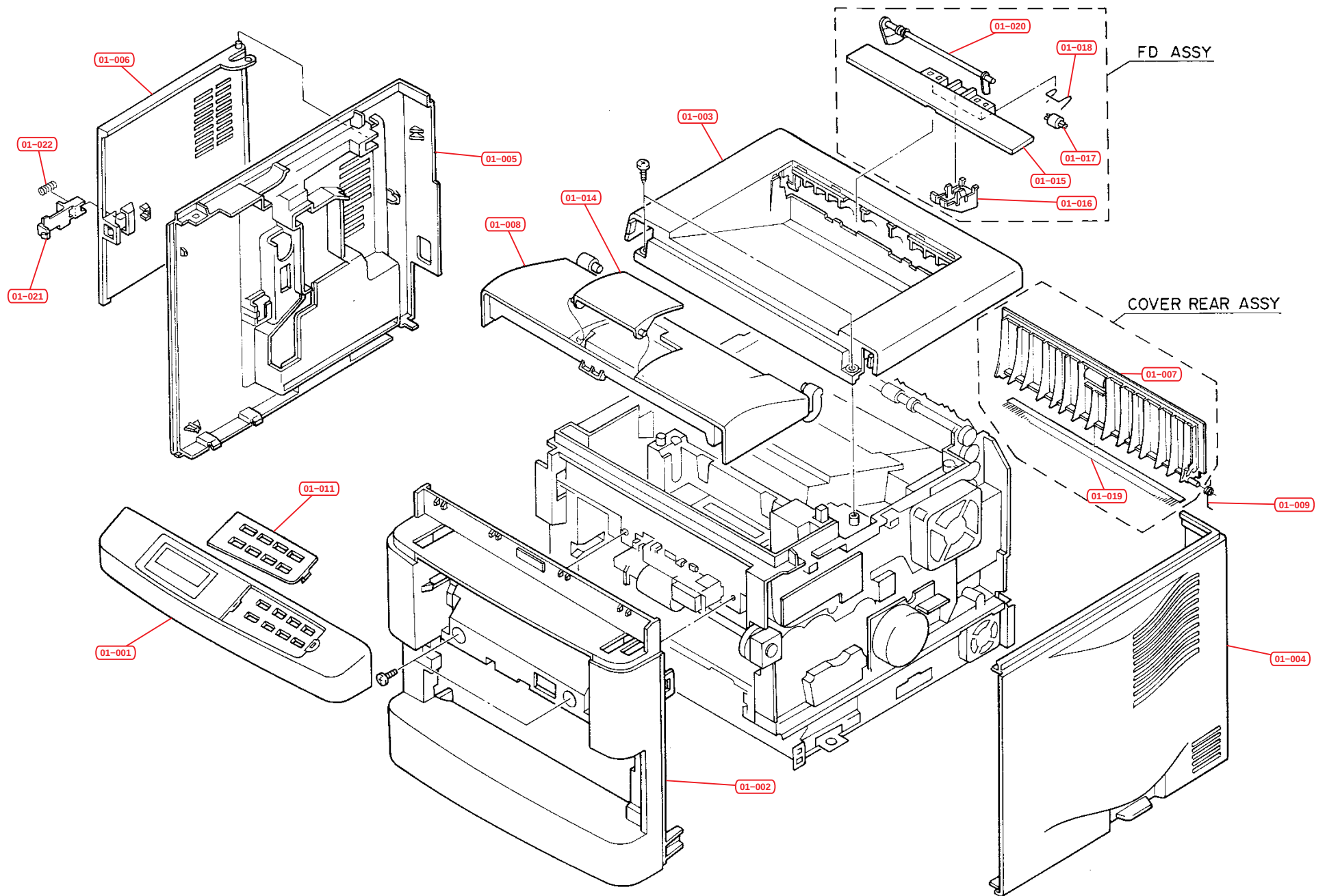
Fig.1 – Covers
