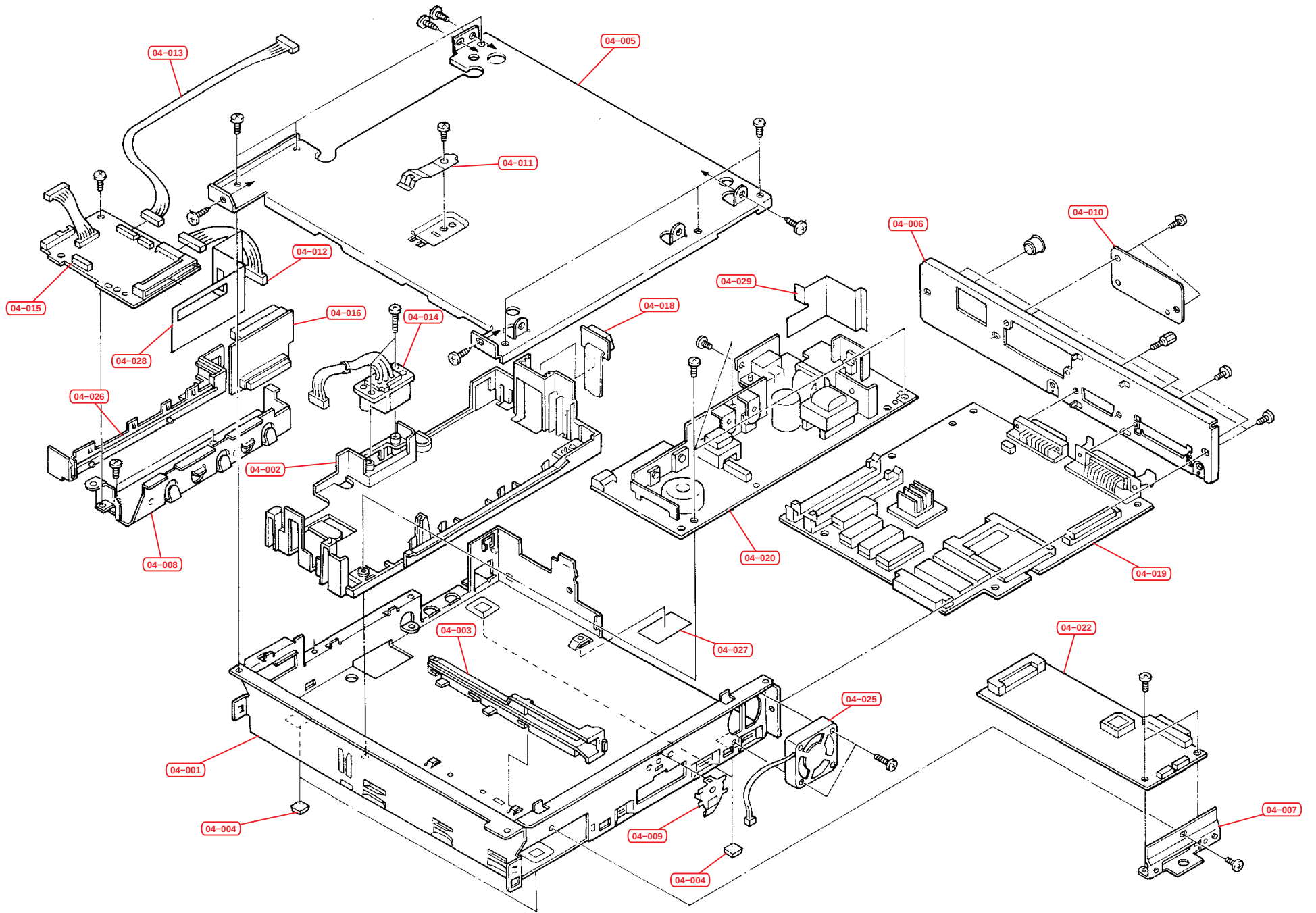
Fig.4 – Controller Unit
