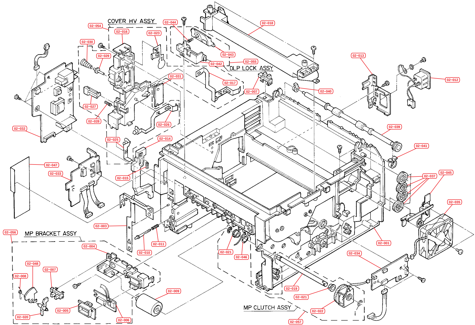
Fig.2 - Frame Unit
