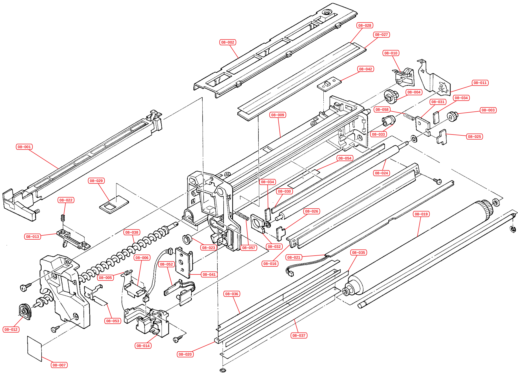
Fig.8 – Drum Unit
