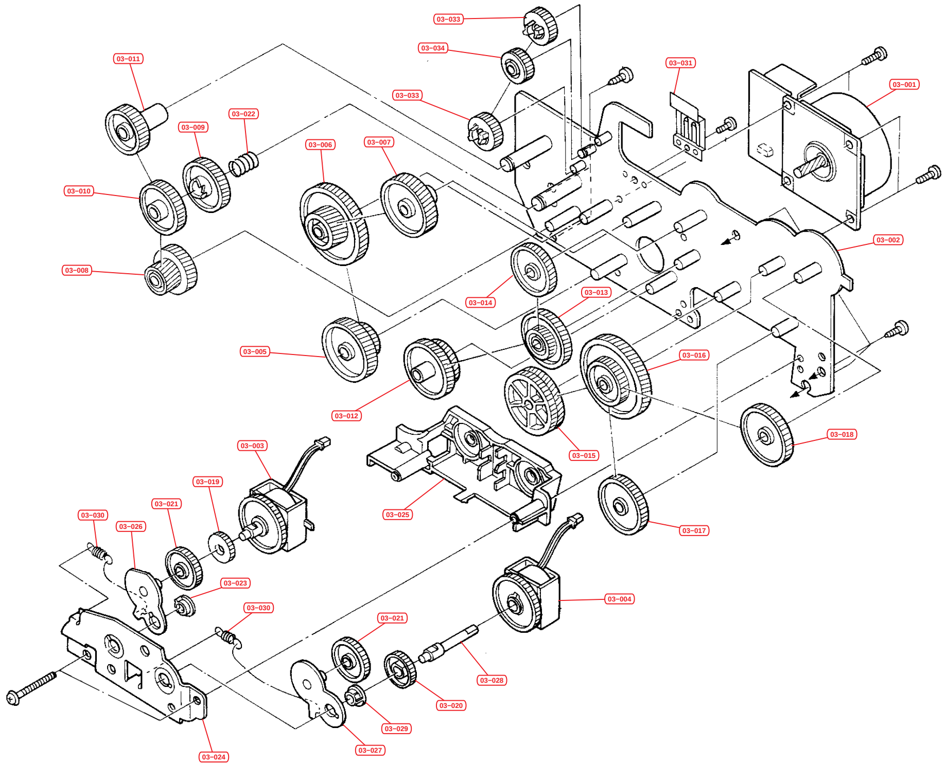
Fig.3 – Drive Unit
