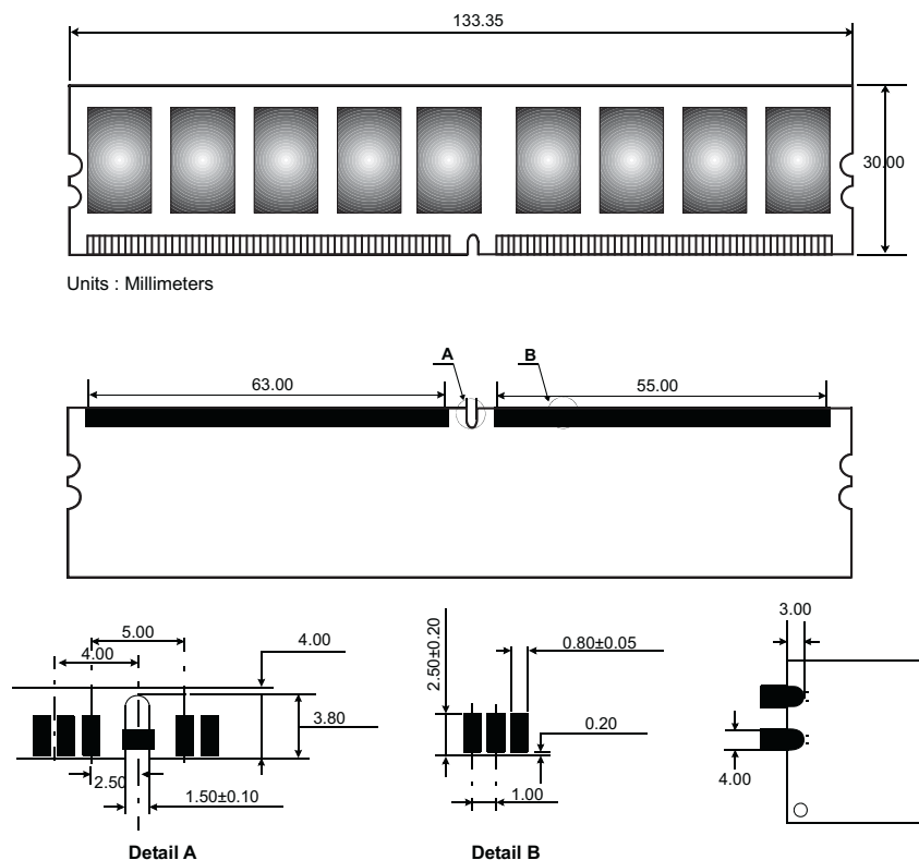
Figure 1: KVR800D2E6/512 240-Pin DIMM
