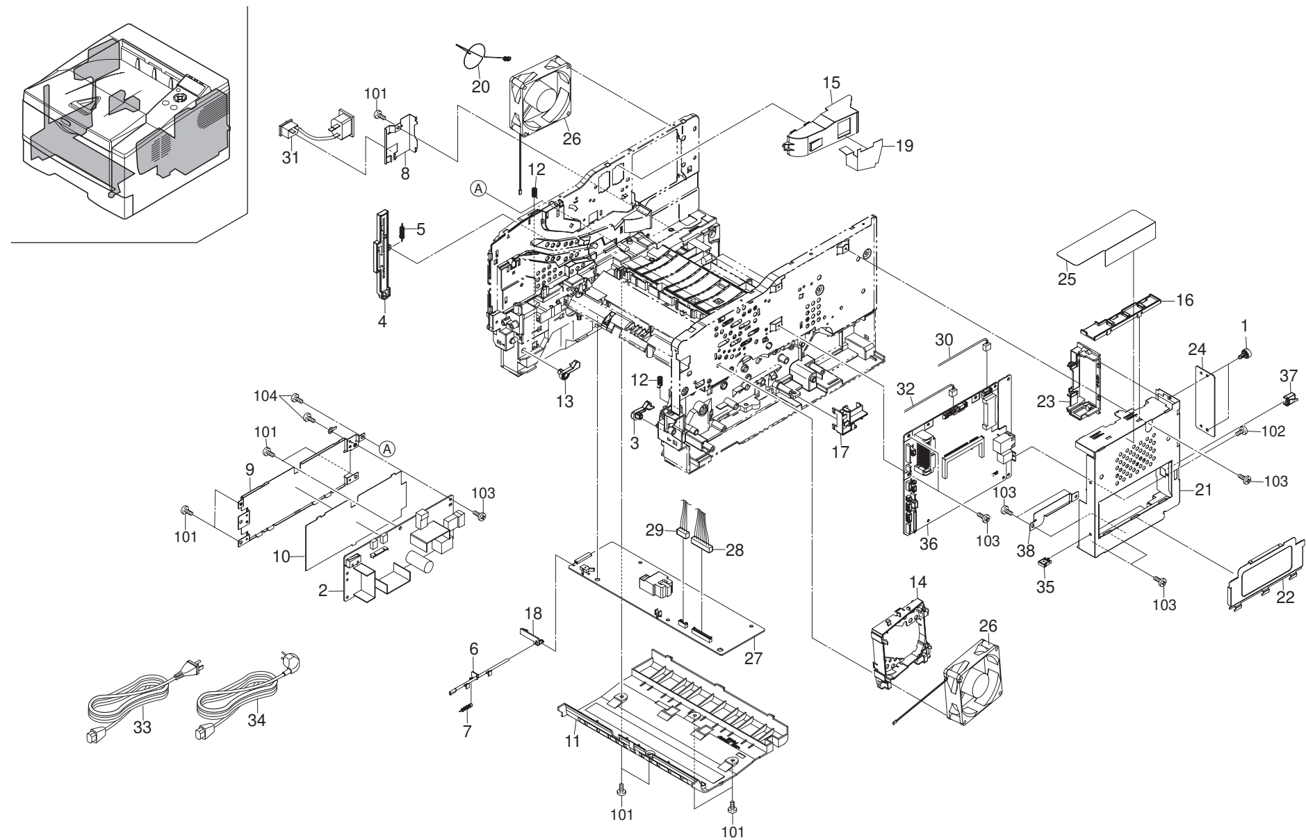
FIG. 11 Electrical Components
