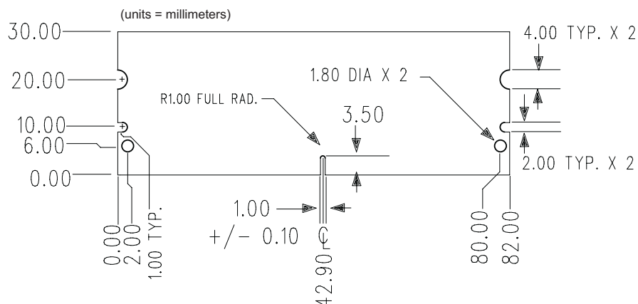
Figure 1: KVR667D2M5/512 244-Pin MiniDIMM
