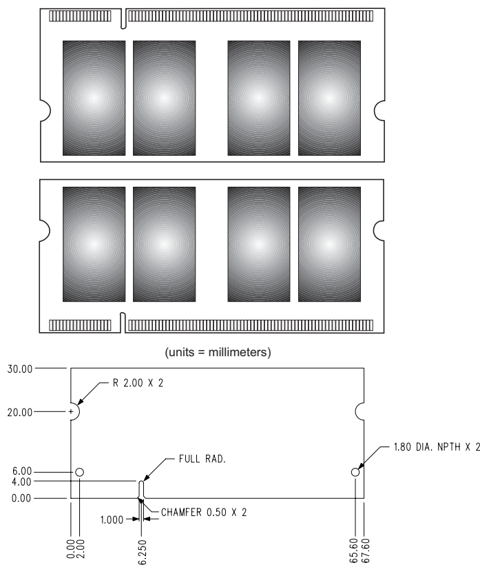
Figure 1: KVR800D2S6K2/1G 200-Pin SODIMM
