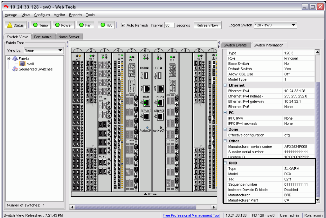
FIGURE 46 Switch RNID information
