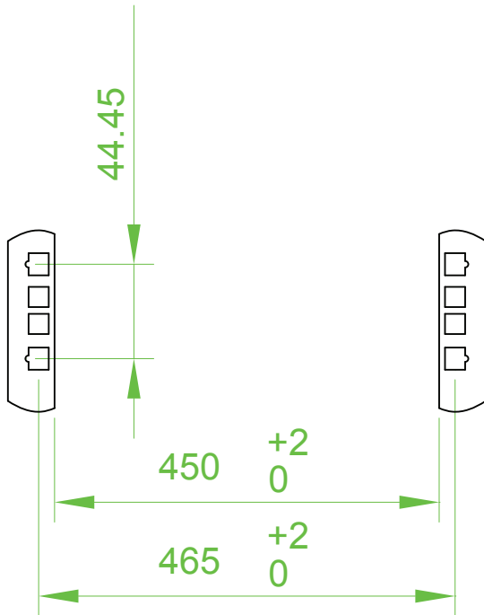
Installation dimension
