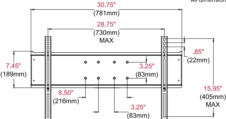
ADAPTOR DETAIL
