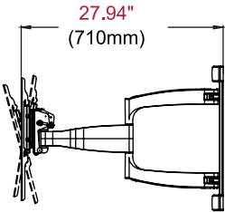
SIDE VIEW EXTENDED +15°/-5° TILT
