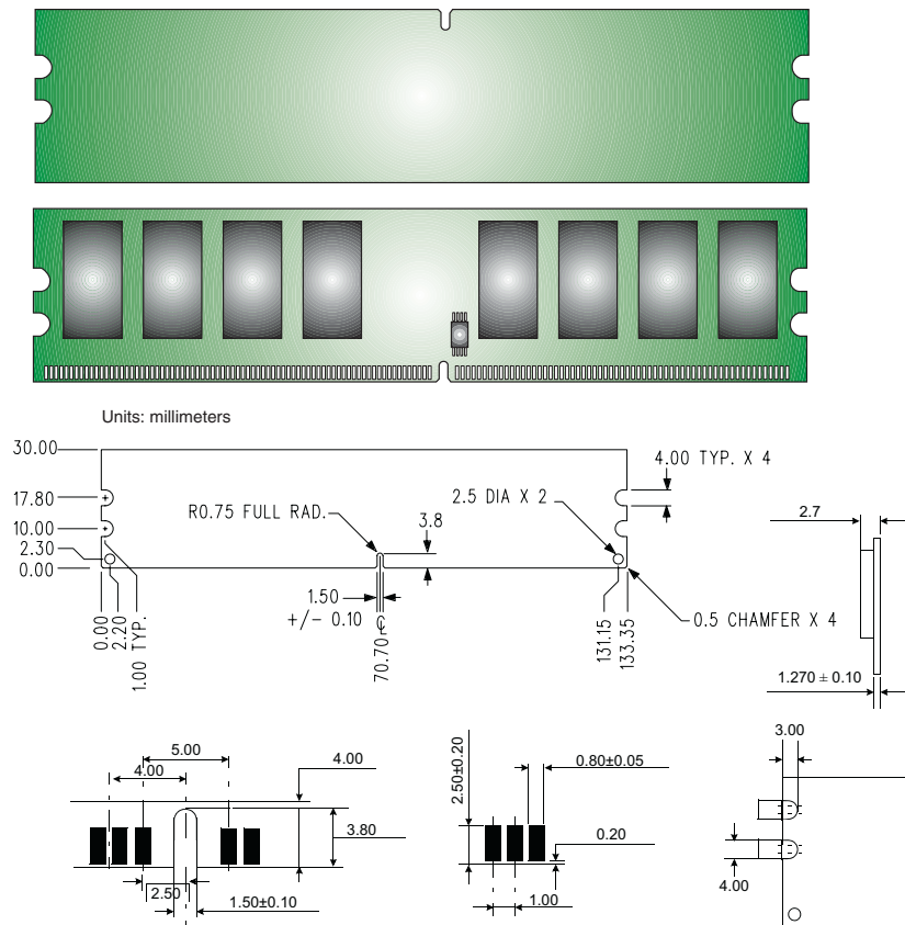
Figure 1: KVR1066D2N7/512 240-Pin DIMM
