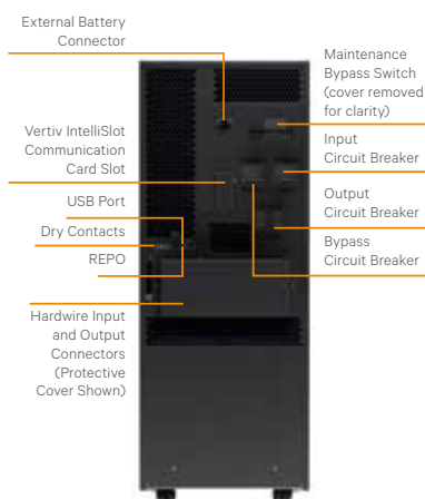
Liebert GXT3-10000T220
