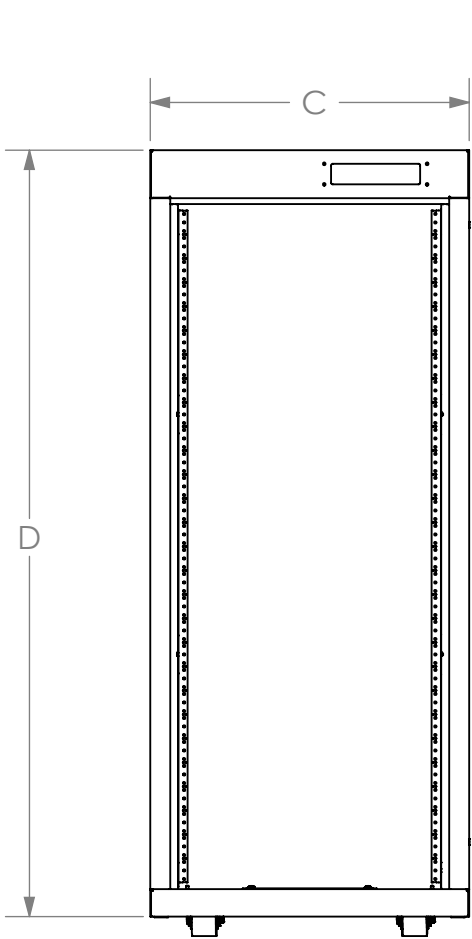
FRONT VIEW
