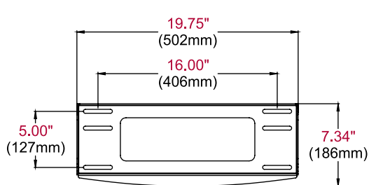
WALL PLATE
