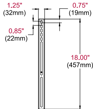
ADAPTOR BRACKET
