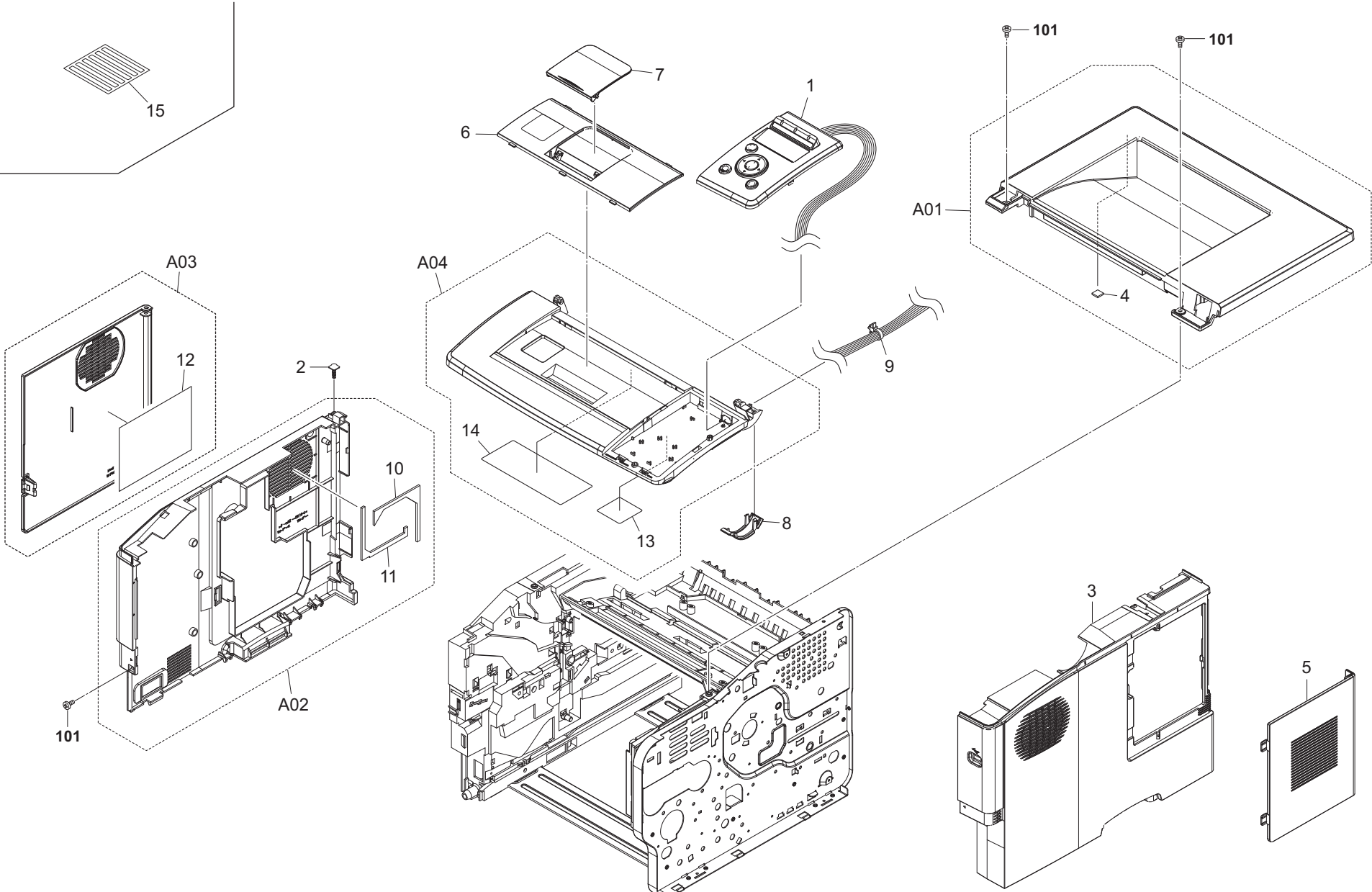
FIG. 1 Covers (FS-2020D)
