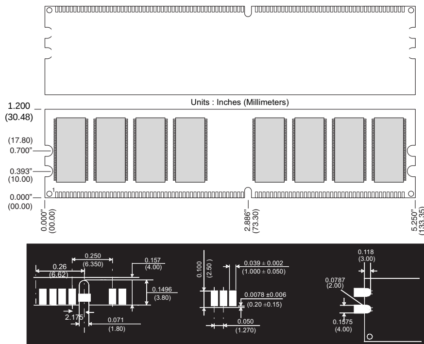
Figure 1: KVR333/256R 184-Pin DIMM
